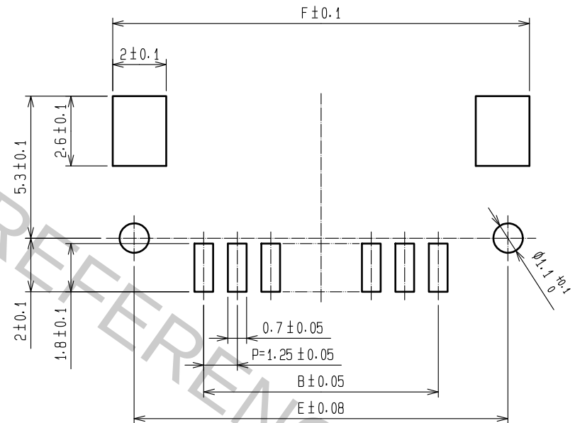
RECOMMENDED PATTERN
