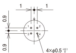
Size 7, 4 conductors
