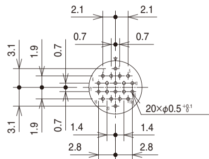
Size 9, 20 conductors
