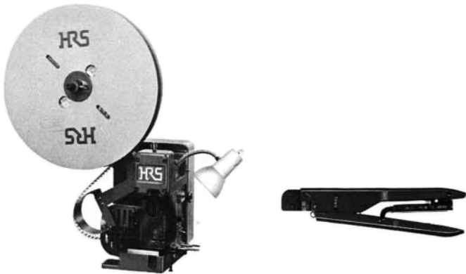
Semi-Auto Machine CM-105 (CL901-0005-4) Applicator (Die) 105-DN50 (CL901-0208-1)
