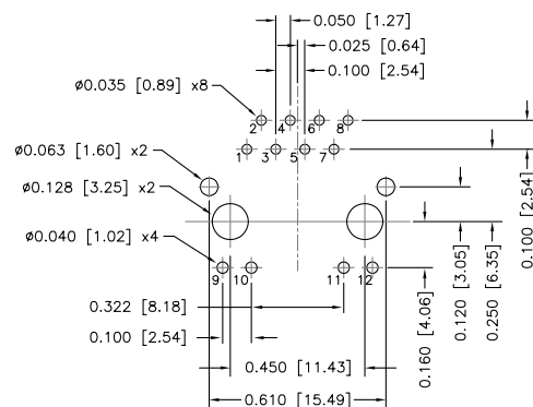
Recommended PCB Layout for Parts with LED (Component Side)
