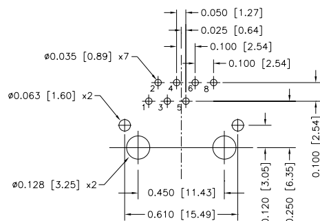
Recommended PCB Layout for Parts without LED (Component Side)
