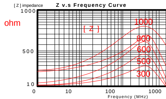
GBD[B] Series [Z] Value Curve
