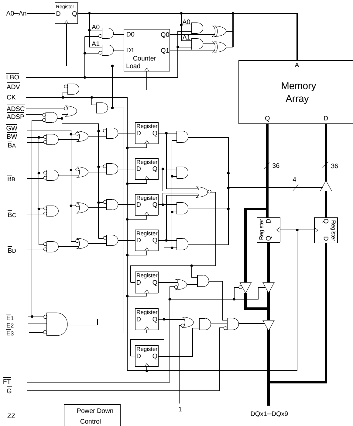
GS88118/32/36C(T/D)-xxxIV Block Diagram
