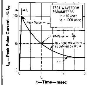
FIGURE 3—Pulse Waveform
