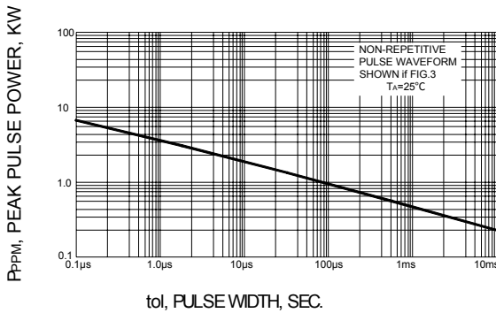
FIG.3 -- PULSE WAVEFORM
