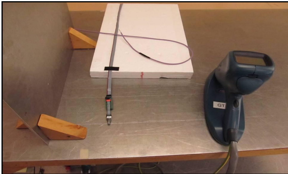
Figure 9 – Electrostatic Discharge Test Setup (Powered)
