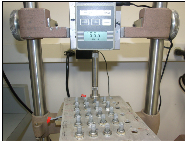
Figure 2– Push Out Force Setup
