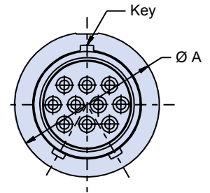
Accessory Thread 804-027-06
