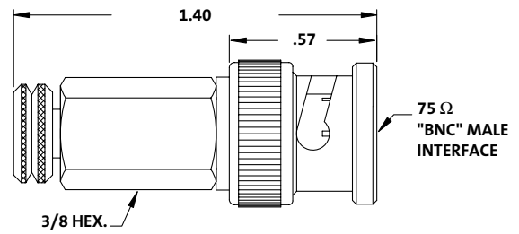
BNC terminator
