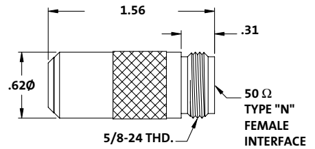
Precision Lab Grade 50Ω N Terminator
