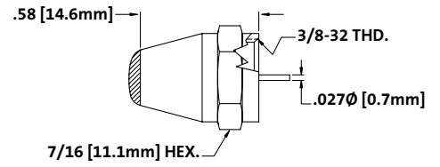
Precision Lab Grade 75Ω ¼ Watt Terminator
