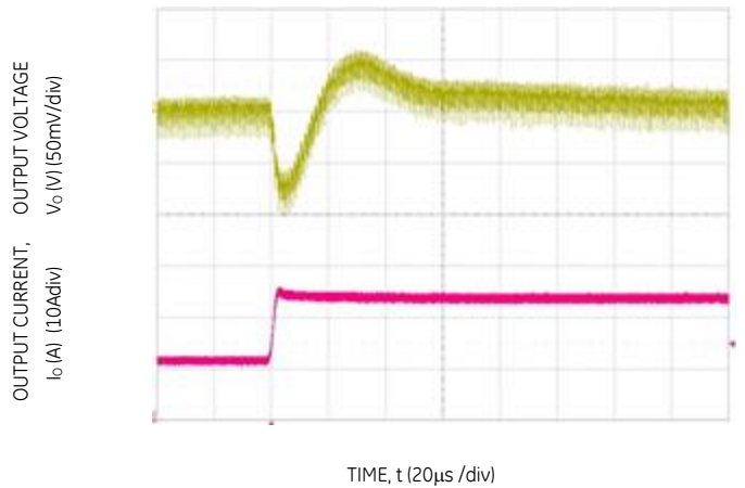
Figure 28. Transient Response to Dynamic Load Change from 50% to 100% at 12V in , C out = 2x47µF+1x330µF, C Tune =2700pF & R Tune =300Ω
