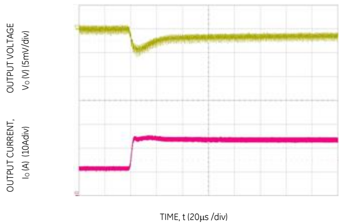
Figure 4. Transient Response to Dynamic Load Change from 50% to 100% at 12Vin, C_{out}=1 \times 47\mu\text{F}+11 \times 330\mu\text{F} , C_{Tune}=47\text{nF} , R_{Tune}=180\Omega
