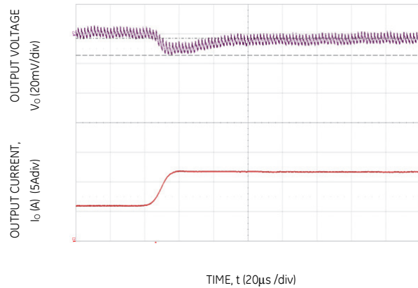
Figure 4. Transient Response to Dynamic Load Change from 50% to 100% on one output at 12Vin, Cout=2x47µF+7x330µF, CTune=12nF, RTune=300Ω
