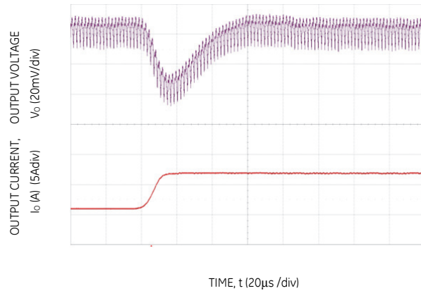
Figure 16. Transient Response to Dynamic Load Change on one output from 50% to 100% at 12V in , C out = 3×47µF+2×330µF, C Tune = 1800pF & R Tune = 300Ω
