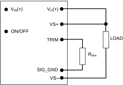
Caution – Do not connect SIG_GND to GND elsewhere in the layout Figure 41. Circuit configuration for programming output voltage using an external resistor.
