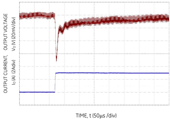
Figure 34. Transient Response to Dynamic Load Change from 50% to 100% at 12Vin, Cout-3x100μF, Ctune-1.5nF, Rtune-500
