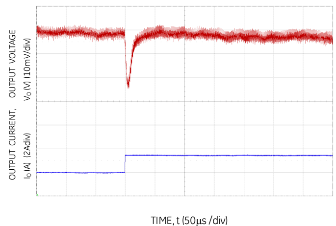
Figure 16. Transient Response to Dynamic Load Change from 50% to 100% at 12Vin, C_{out}=4\times 100\mu\text{F} , C_{tune}=4.7\text{nF} , R_{tune}=400
