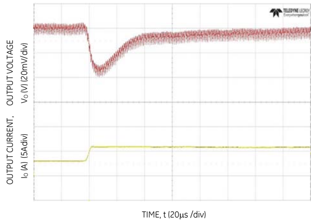
Figure 22. Transient Response to Dynamic Load Change from 50% to 100% at 12Vin, C_{out}=3 \times 47 \mu F + 1 \times 330 \mu F , C_{Tune}=2200pF , R_{Tune}=300 \Omega
