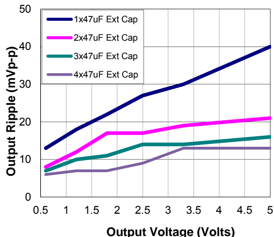
Figure 38. Output ripple voltage for various output voltages with external 1x47μF, 2x47 μF, 3x47 μF, or 4x47 μF ceramic capacitors at the output (6A load). Input voltage is 12V. Scope BW Limited to 20MHz
