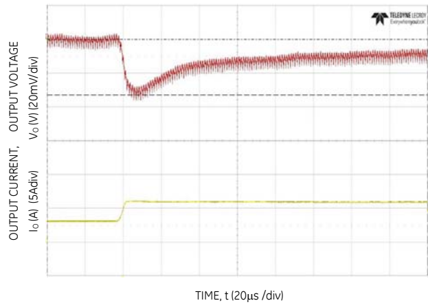
Figure 16. Transient Response to Dynamic Load Change from 50% to 100% at 12Vin, C_{out}=3 \times 47 \mu F + 1 \times 330 \mu F , C_{Tune}=3900pF , R_{Tune}=300
