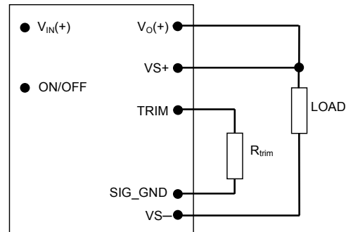
Caution – Do not connect SIG_GND to GND elsewhere in the layout
