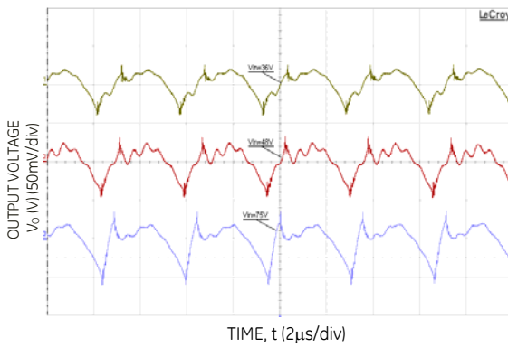
Figure 2. Typical output ripple and noise ( I_o = I_{o,max} ).
