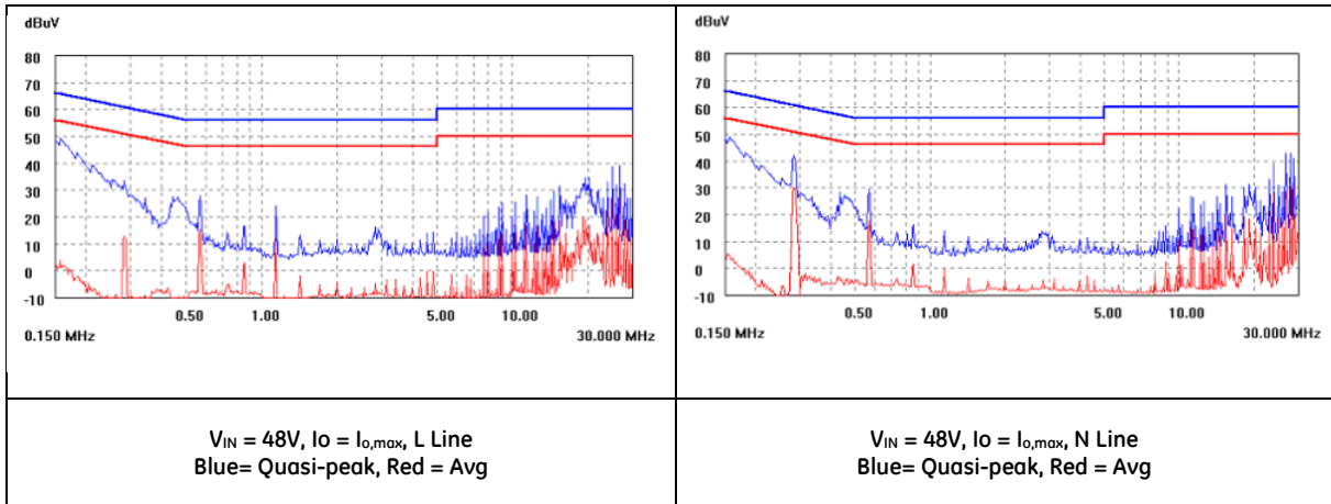
Figure 25. EMC Considerations.
