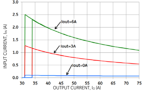
Figure 2. Input Current versus Output Current.
