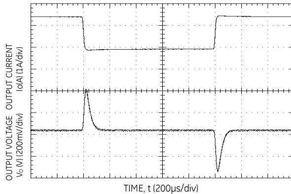
Figure 5. Transient Response to 0.1A/µS Dynamic Load Change from 50% to 75% to 50% of full load, V_{in}=48V, C_o>100µF .
