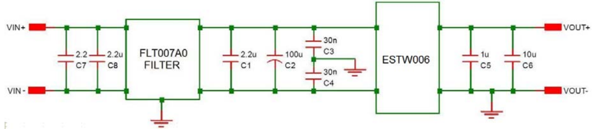
Figure 25. EMC Considerations.
