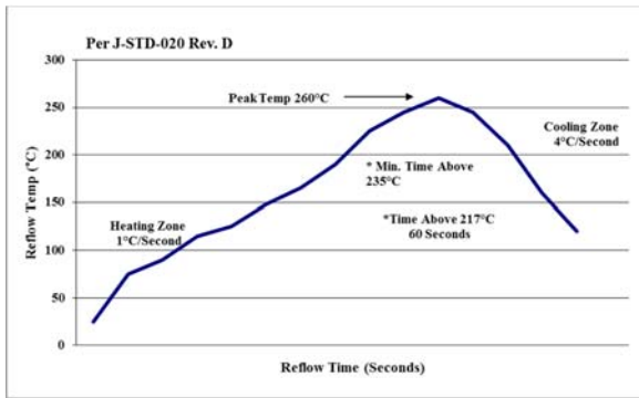
Figure 24. Recommended linear reflow profile using Sn/Ag/Cu solder.
