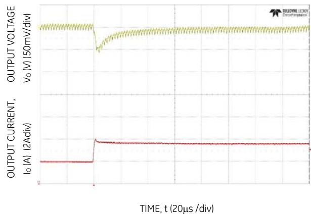
Figure 22. Transient Response to Dynamic Load Change from 50% to 100% at 12Vin, Cout=3x47µF, CTune=1.5nF, RTune=300
