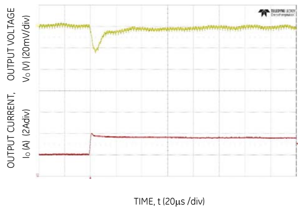
Figure 10. Transient Response to Dynamic Load Change from 50% to 100% at 12Vin, Cout=8x47uF, CTune=4.7nF, RTune=300
