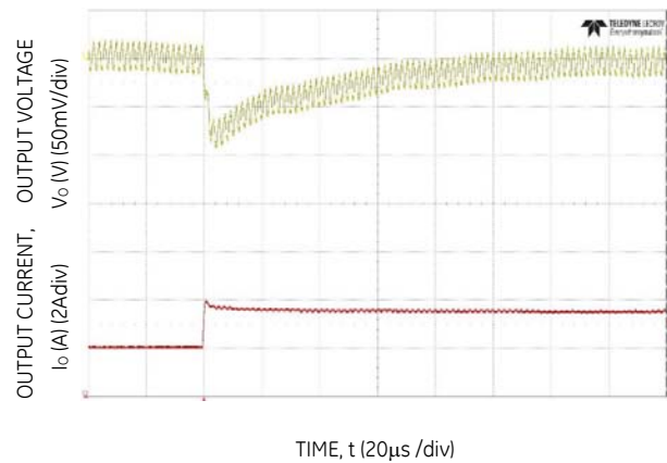
Figure 34. Transient Response to Dynamic Load Change from 50% to 100% at 12V in , C out =2x47µF, C Tune =220pF, R Tune =300
