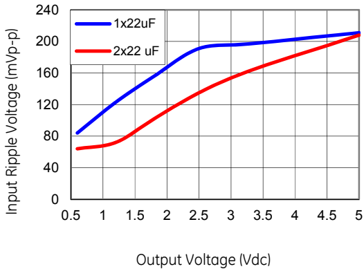
Figure 37. Input ripple voltage for various output voltages with 1x22 \mu F or 2x22 \mu F ceramic capacitors at the input (4A load). Input voltage is 12V.
