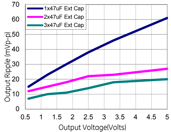
Figure 38. Output ripple voltage for various output voltages with external 1x47 \mu F, 2x47 \mu F or 3x47 \mu F ceramic capacitors at the output (4A load). Input voltage is 12V.
