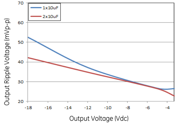
Figure 68. Output ripple with 1x10µF or 2x10µF output ceramic capacitors (max load).
