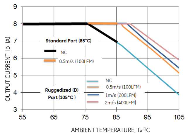
Figure 55. Derating Output Current versus Ambient Temperature and Airflow.
