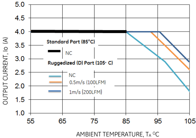
Figure 58. Derating Output Current versus Ambient Temperature and Airflow.
