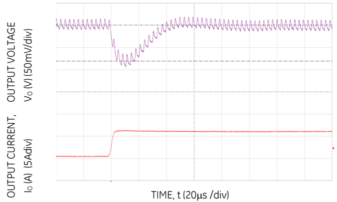
Figure 10. Transient Response to Dynamic Load Change from 50% to 100% at 28Vin, C_{ext} = 1 \times 22\mu F + 1 \times 330\mu F , C_{Tune} = 5.6nF & R_{Tune} = 200
