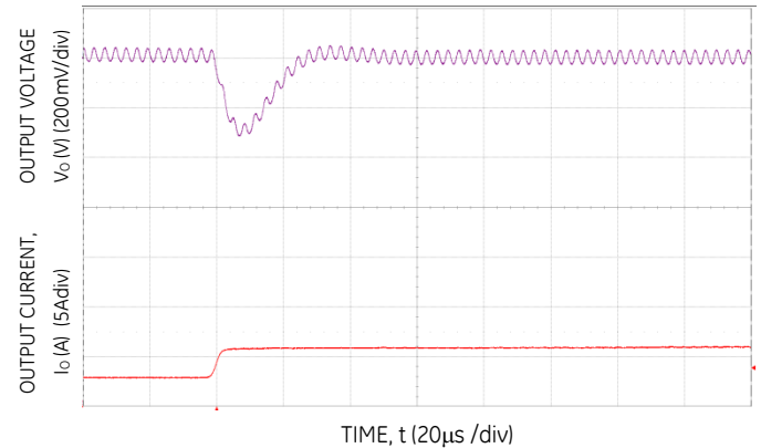
Figure 22. Transient Response to Dynamic Load Change from 50% to 100% at 28Vin, C_{ext} = 5 \times 22\mu F , C_{Tune} = 220pF & R_{Tune} = 200
