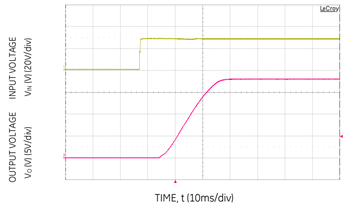
Figure 24. Typical Start-up Using Input Voltage ( V_{IN} = 28V , I_o = I_{o,max} ).
