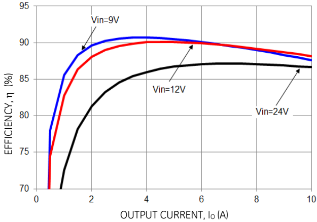
Figure 48. Converter Efficiency versus Output Current.
