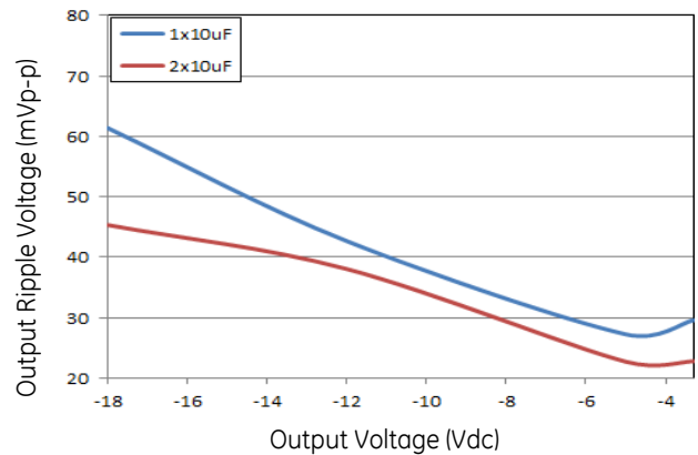
Figure 69. Output ripple with 1x10µF or 2x10µF output ceramic capacitors (max load).
