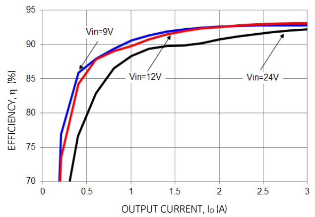
Figure 50. Converter Efficiency versus Output Current.
