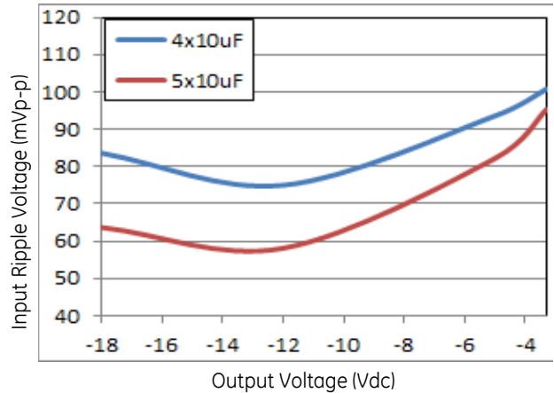
Figure 66. Input ripple voltage with 4x10 μF or 5x10 μF input ceramic capacitors (max load).
