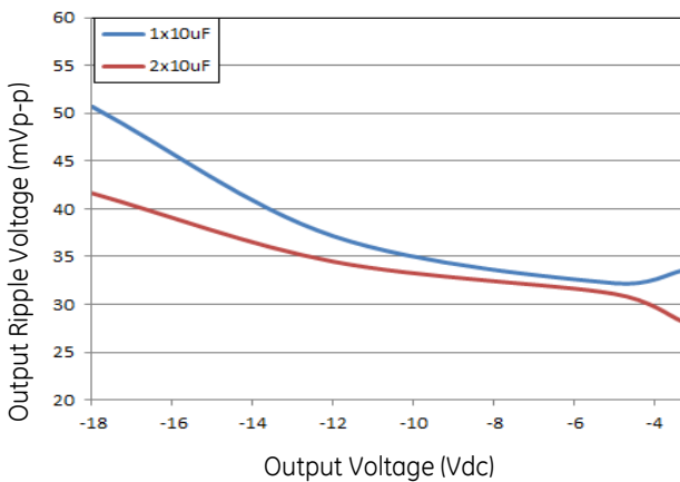
Figure 67. Output ripple with 1x10µF or 2x10µF output ceramic capacitors (max load).
