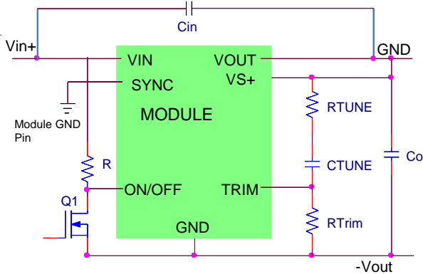
Figure 45. Schematic Connection of 12A ProLynx module for negative output applications.
