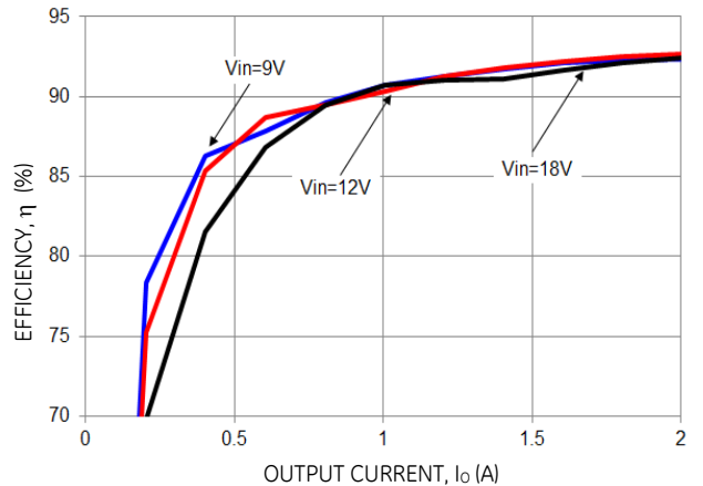
Figure 51. Converter Efficiency versus Output Current.
