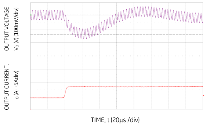
Figure 16. Transient Response to Dynamic Load Change from 50% to 100% at 28Vin, C_{ext} = 1x22\mu F + 1x470\mu F , C_{Tune} = 1.5nF & R_{Tune} = 200
