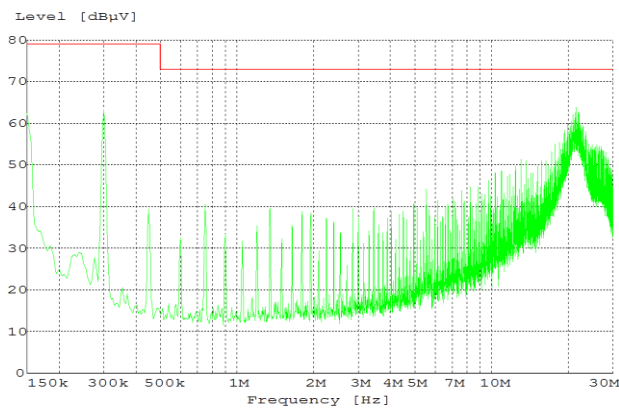
Figure 25. EMC Consideration
