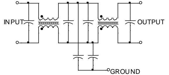
Figure 4. Internal Schematic
