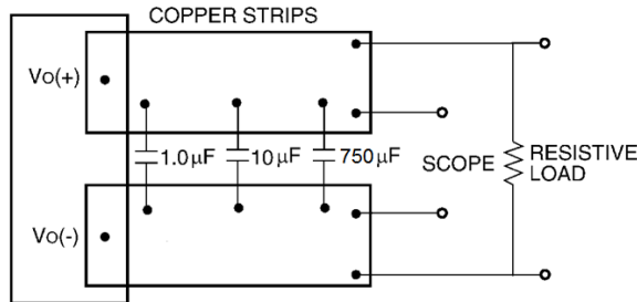
Figure 13. Input Reflected Ripple Current Test Setup.
