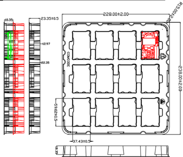
Base Plate Module Tray Figure 27. QBDE067A0B Packaging Tray
