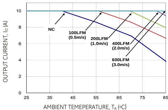
Figure 19. Output Current Derating for the Module with Heatplate; Airflow in the Transverse Direction from V out (-) to V out (+); V IN =24V, V O =12V.
