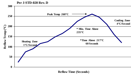
Figure 26. Recommended linear reflow profile using Sn/Ag/Cu solder.
