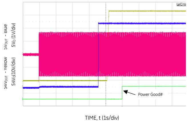
Figure 14. Turn-ON at full load V_{IN} = 230V_{AC} .
