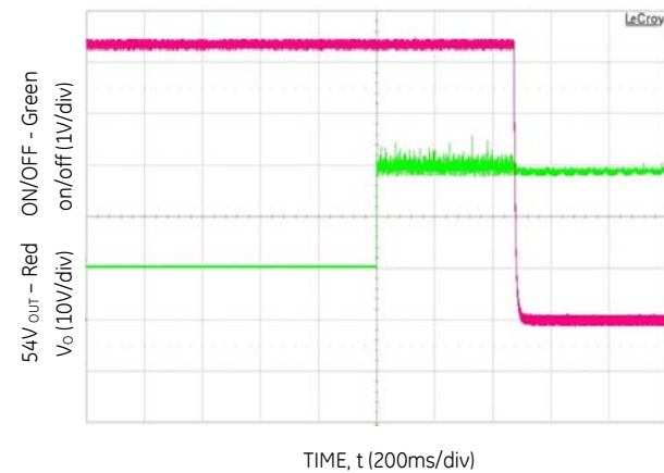
Figure 16. 54V DC turn-OFF delay when ON/OFF is disasserted, V_{IN}=230V_{AC} - I 2 C mode.
