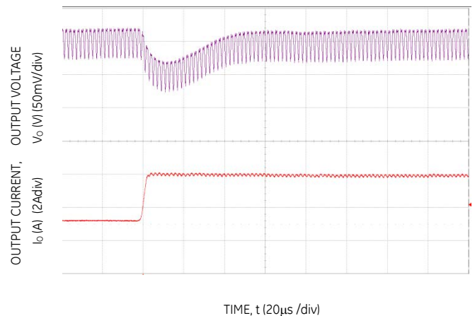
Figure 28 Transient Response to Dynamic Load Change on one output from 50% to 100% at 12V in , C_{out} = 2 \times 47\text{uF} + 1 \times 330\text{uF} , C_{Tune} = 1200\text{pF} & R_{Tune} = 300\Omega
