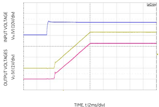
Figure 30. Typical Start-up Using Input Voltage ( V_{in} = 12\text{V} , I_o = I_{o1,max}, I_{o2,max} ).
