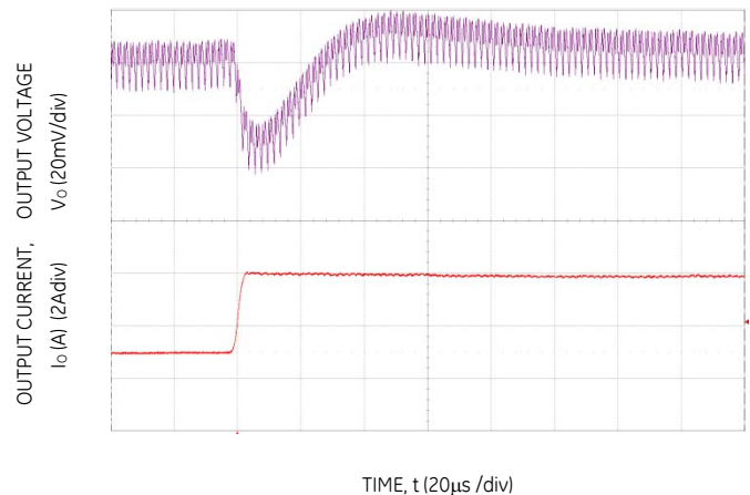
Figure 16. Transient Response to Dynamic Load Change on one output from 50% to 100% at 12Vin, C_{out} = 3 \times 47\text{uF} + 1 \times 330\text{uF} , C_{Tune} = 1800\text{pF} & R_{Tune} = 300\Omega
