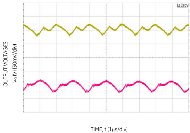
Figure 21. Typical output ripple and noise ( C_o = 2 \times 4.7\text{nF} + 2 \times 47\text{uF} ceramic, V_{in} = 12\text{V} , I_o = I_{o1,max}, I_{o2,max} ).
