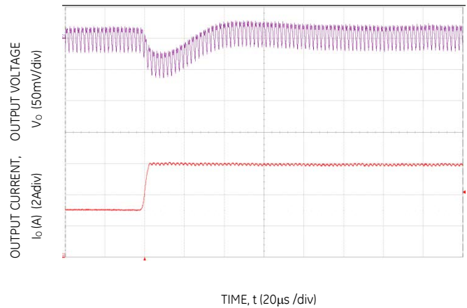
Figure 22. Transient Response to Dynamic Load Change on one output from 50% to 100% at 12V in , C_{out} = 2 \times 47\text{uF} + 1 \times 330\text{uF} , C_{Tune} = 1500\text{pF} & R_{Tune} = 300\Omega
