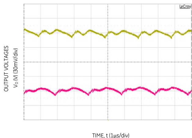
Figure 9. Typical output ripple and noise ( C_o = 2 \times 4.7\text{nF} + 2 \times 47\mu\text{F} ceramic, V_{in} = 12\text{V} , I_o = I_{o1,max}, I_{o2,max} ).
