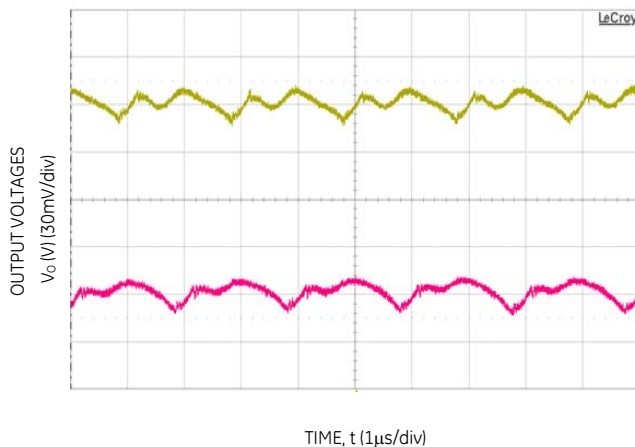
Figure 15. Typical output ripple and noise ( C_o = 2 \times 4.7\text{nF} + 2 \times 47\text{uF} ceramic, V_{IN} = 12\text{V} , I_o = I_{o1,max}, I_{o2,max} ).
