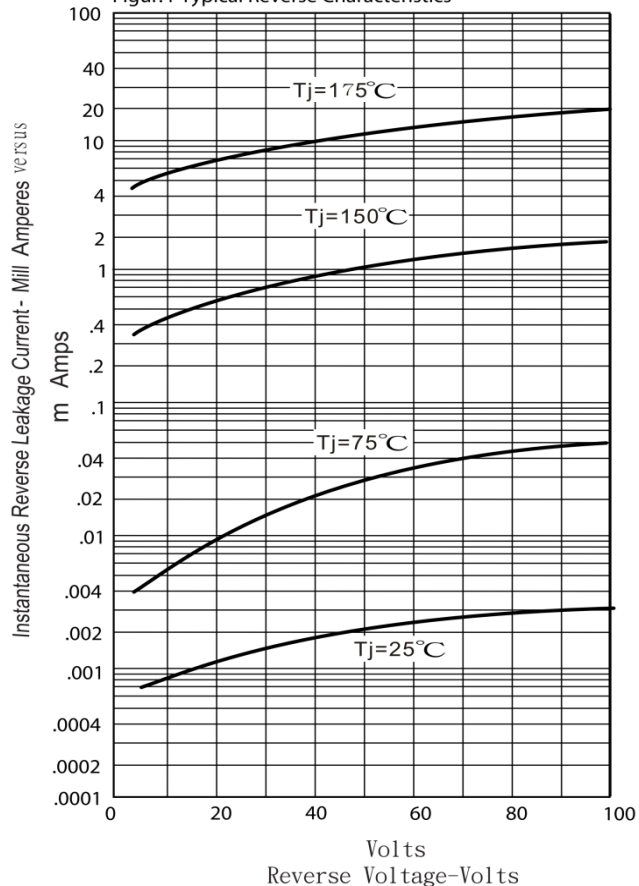
Figure.4-Typical Reverse Characteristics
