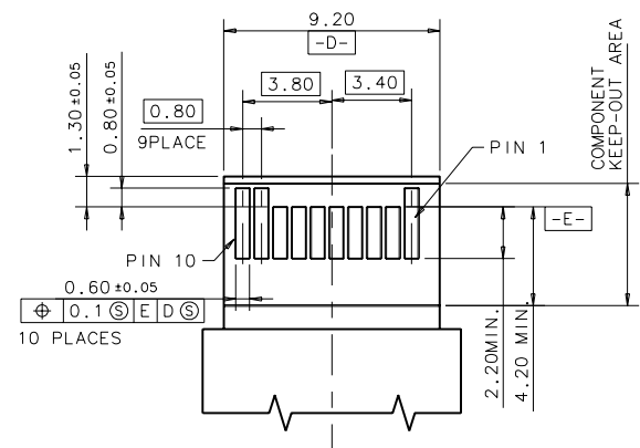
BOTTOM VIEW OF BOARD
