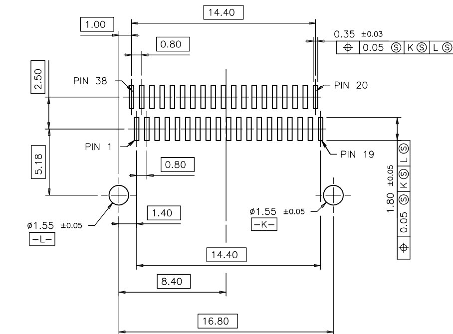
RECOMMENDED PCB LAYOUT FOR 3S10382*-01-7* (COMPONENT SIDE)
