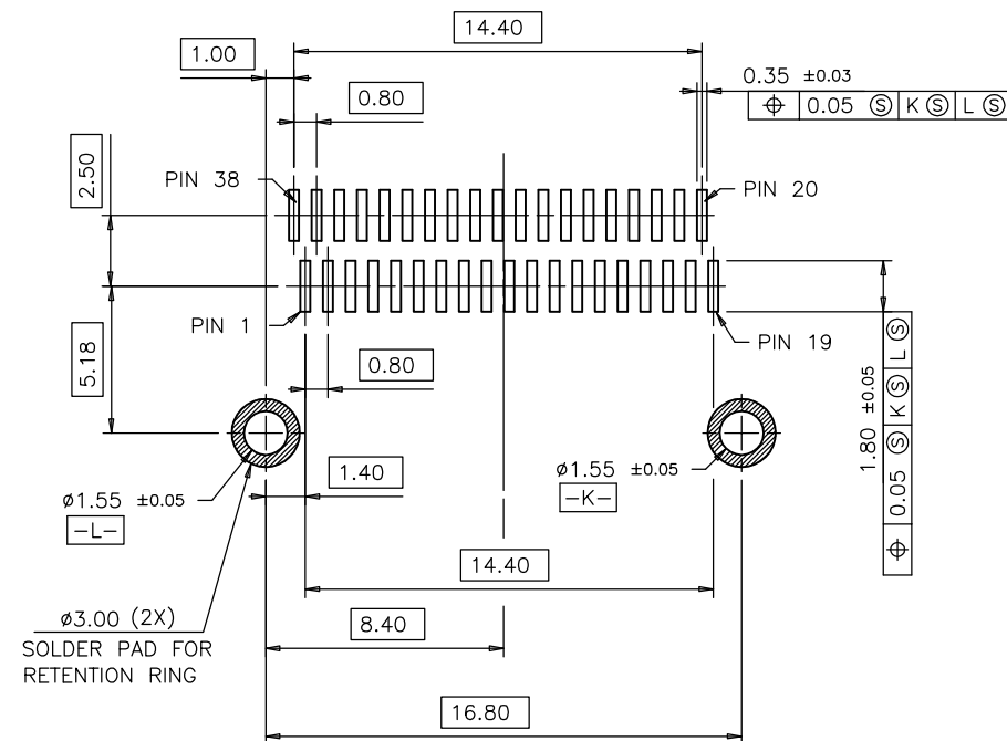
RECOMMENDED PCB LAYOUT FOR 3S3A013-00506-7F (COMPONENT SIDE)
