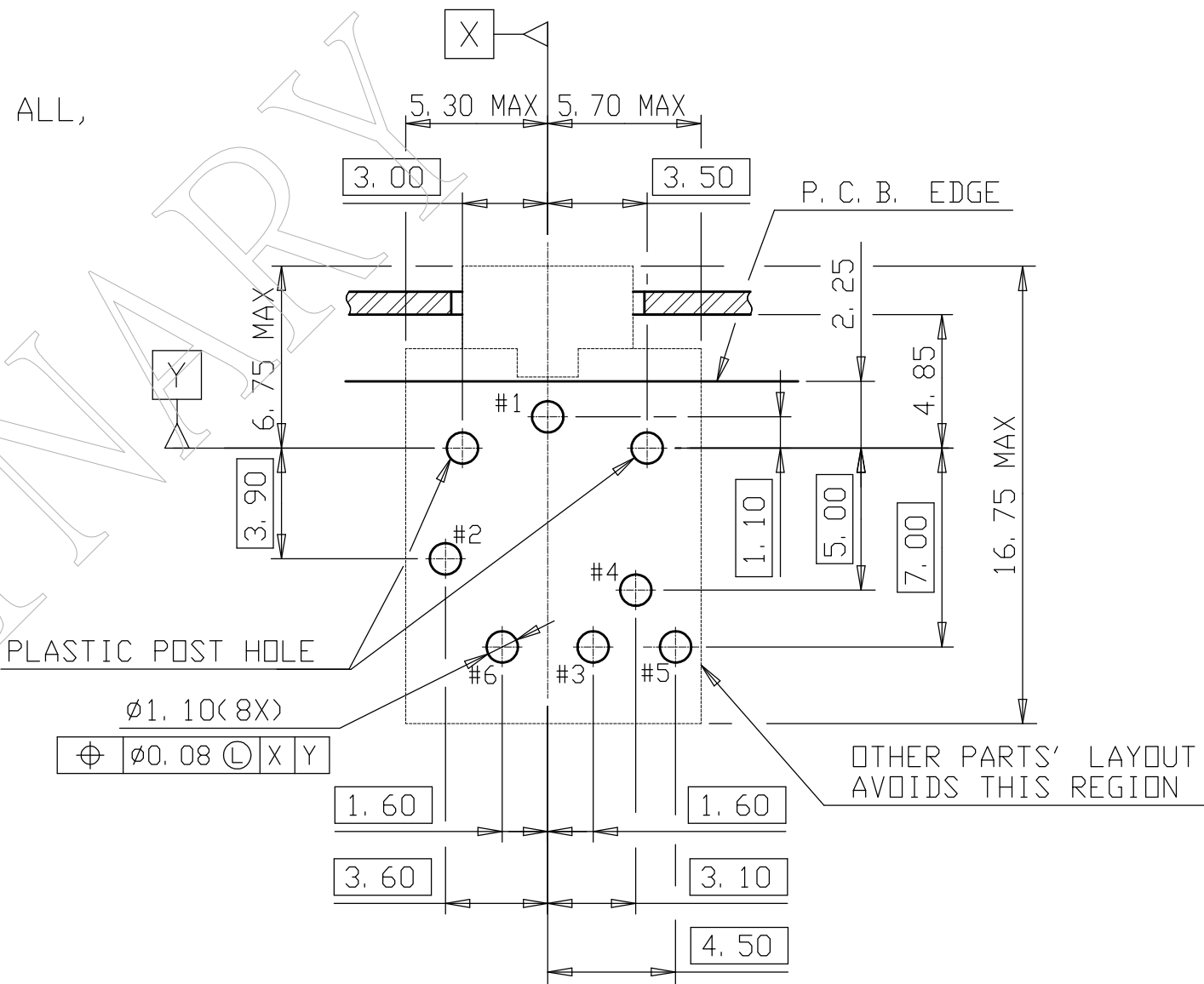
RECOMMENDED P. C. B. LAYOUT (TOP VIEW) (UNSPECIFIED TOLERANCE: ±0.05)
