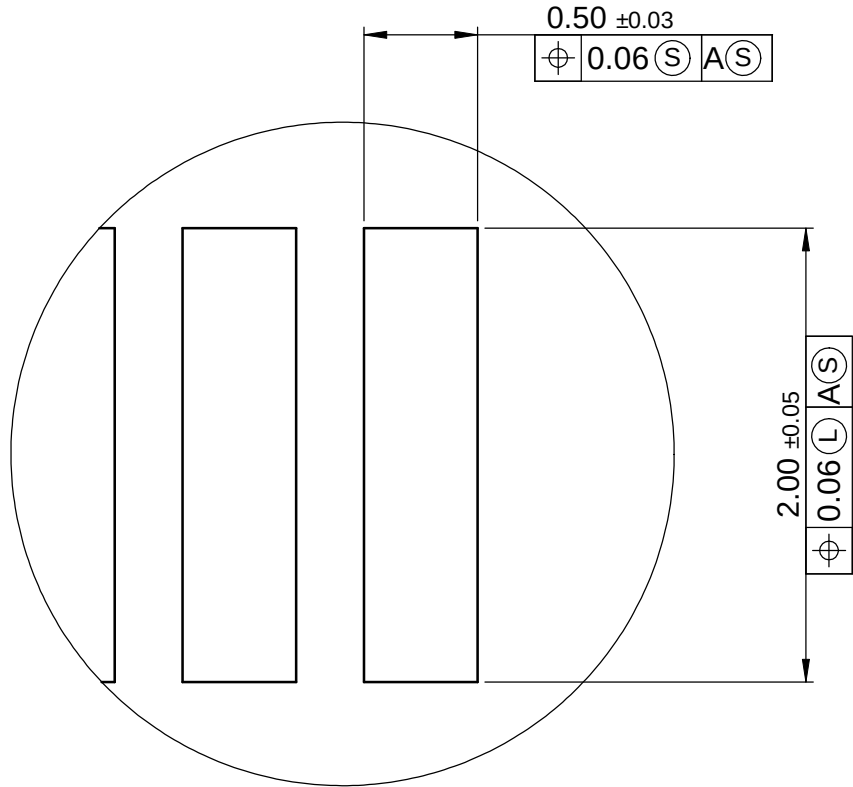
DETAIL C SCALE 30 : 1
