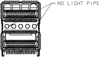
W/O LIGHT PIPE TYPE P/N: 3S1076C3-AG4-4M
