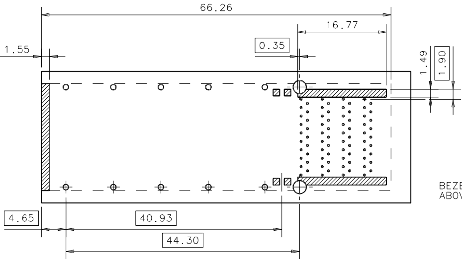
KEEP-OUT AREAS COMPONENT SIDE
