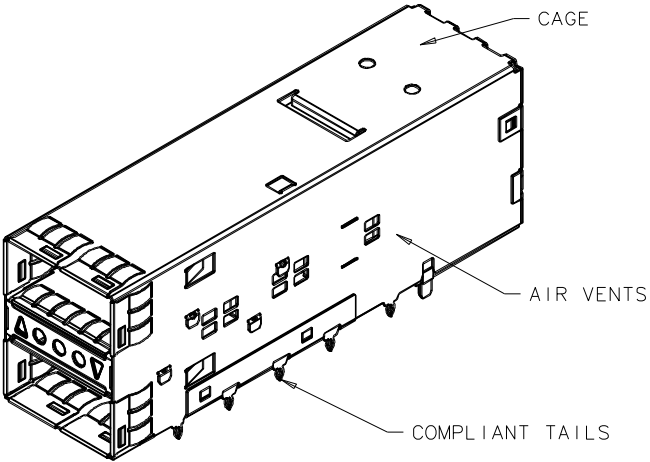
3D VIEW W/ LIGHT PIPE TYPE
