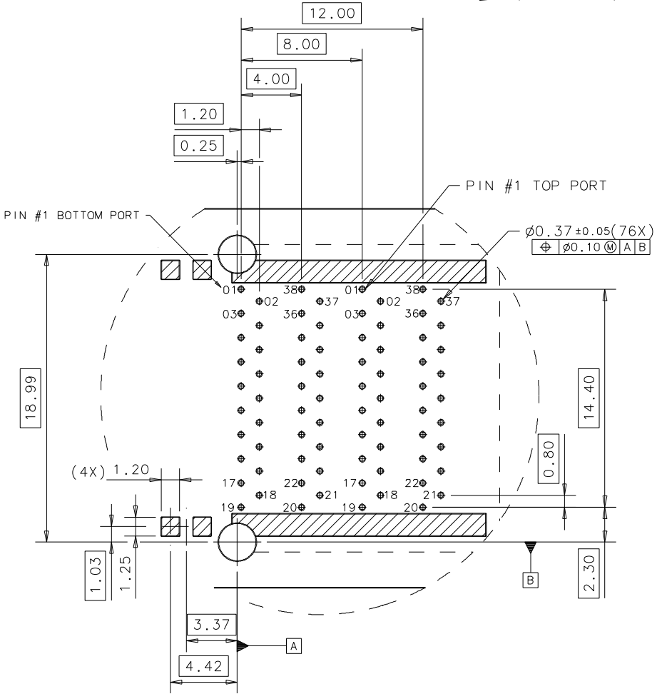
DETAIL B
