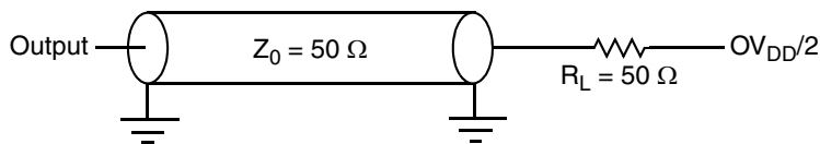
Figure 22. AC Test Load for the JTAG Interface
