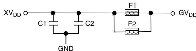
Figure 49. XV_{DD} Power Supply Filter Circuit
