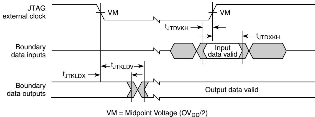
Figure 25. Boundary-Scan Timing Diagram
