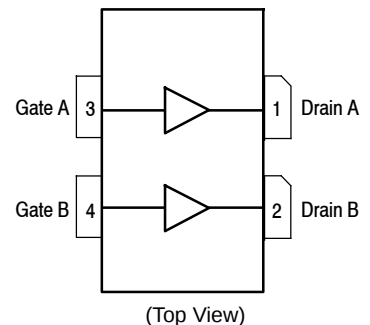
Figure 1. Pin Connections
