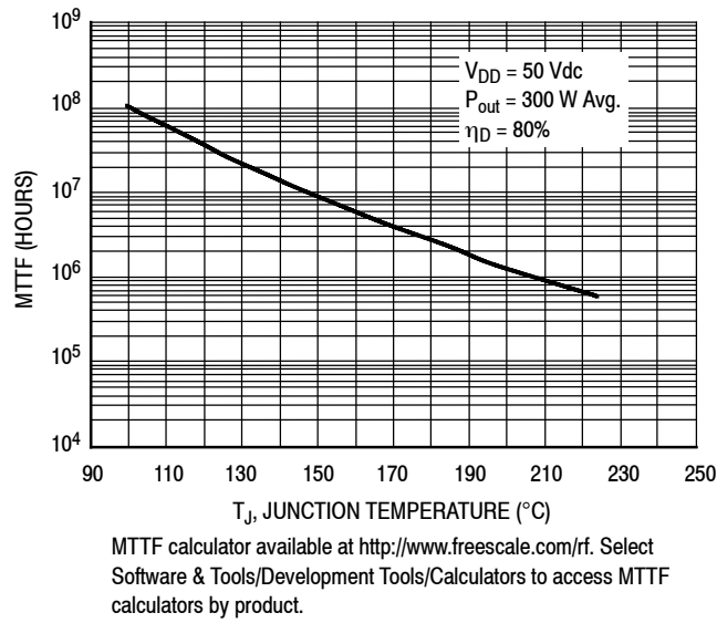
Figure 14. MTTF versus Junction Temperature — CW
