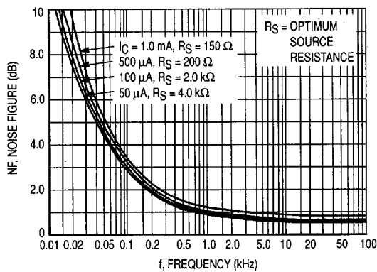
Figure 7. Frequency Effects
