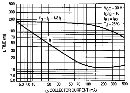
Figure 6. Turn-Off Time
