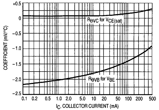
Figure 12. Temperature Coefficients
