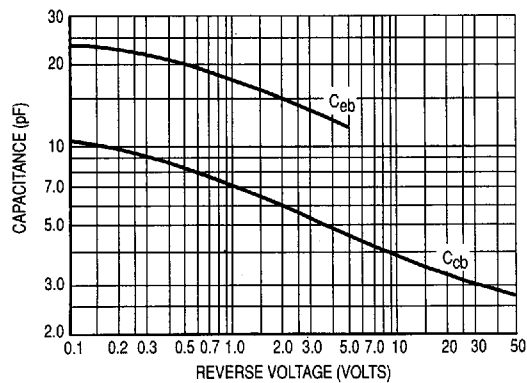
Figure 9. Capacitances
