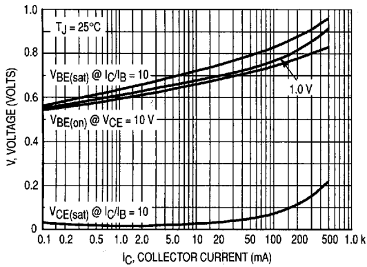
Figure 11. "On" Voltages
