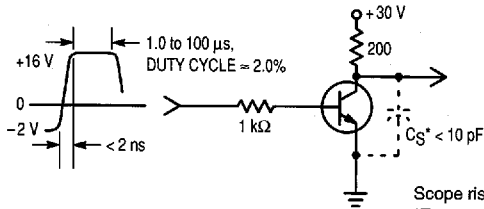
Figure 1. Turn-On Time
