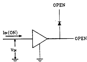
5. V_{IN(ON)}
