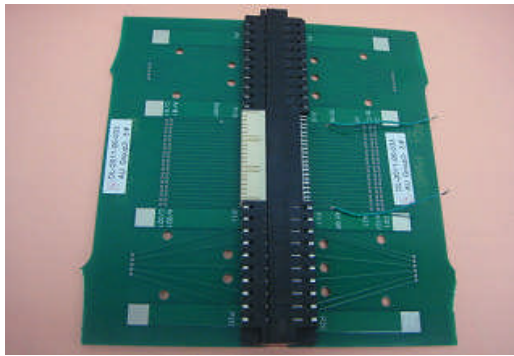
Figure 2 Test sample Consisting of a Mate Pair of PwrBlade® Connectors Mounted on Test Boards
