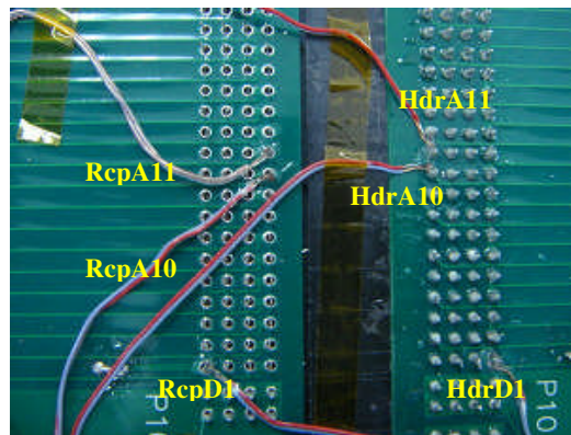
Figure 3 Photo of Thermocouples location
