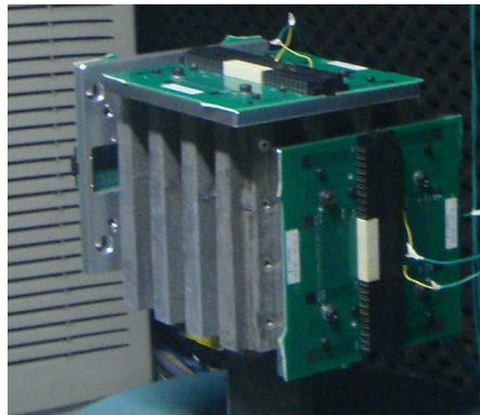
Figure 4 PwrBlade Sample Fixturing for Shock and Vibration testing
