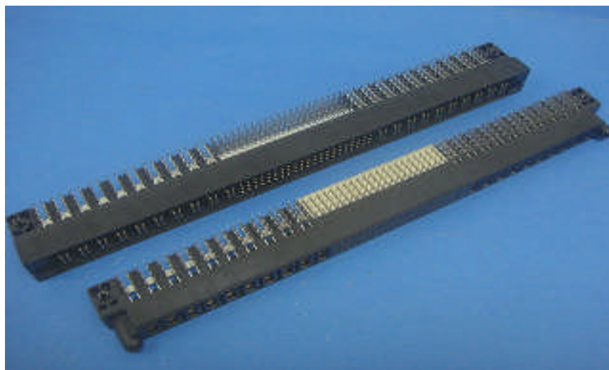
Figure1 Test sample- PwrBlade® R/A Header and Receptacle
