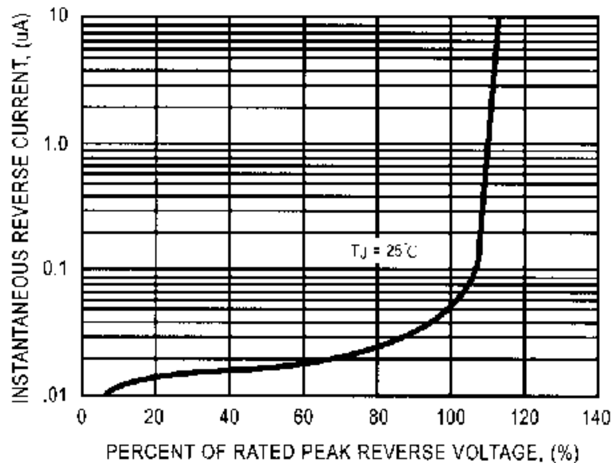
FIG. 4 - TYPICAL REVERSE CHARACTERISTICS
