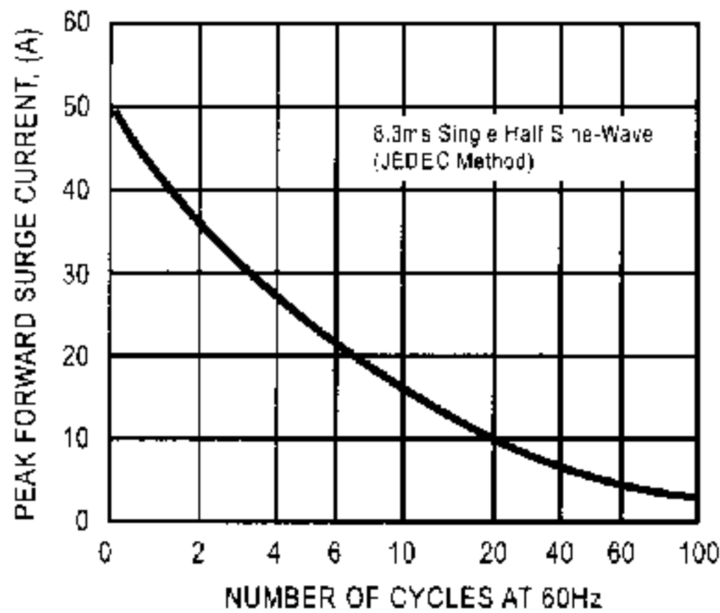
FIG. 1 - MAXIMUM NON-REPETITIVE FORWARD SURGE CURRENT
