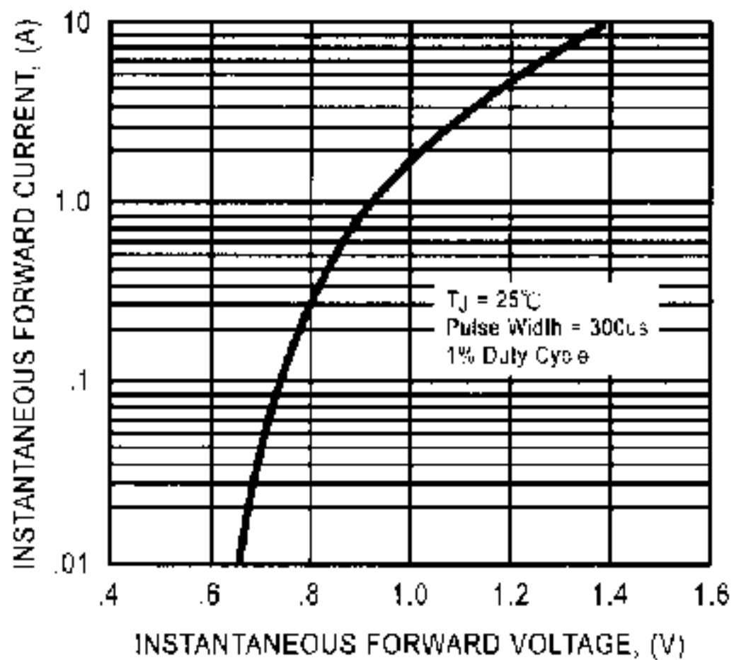
FIG. 3 - TYPICAL INSTANTANEOUS FORWARD CHARACTERISTICS
