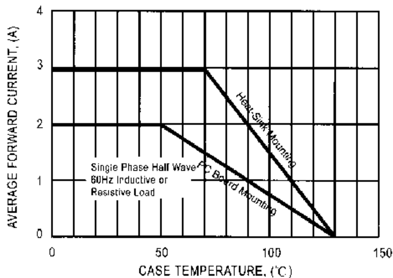
FIG. 2 - TYPICAL FORWARD CURRENT DERATING CURVE
