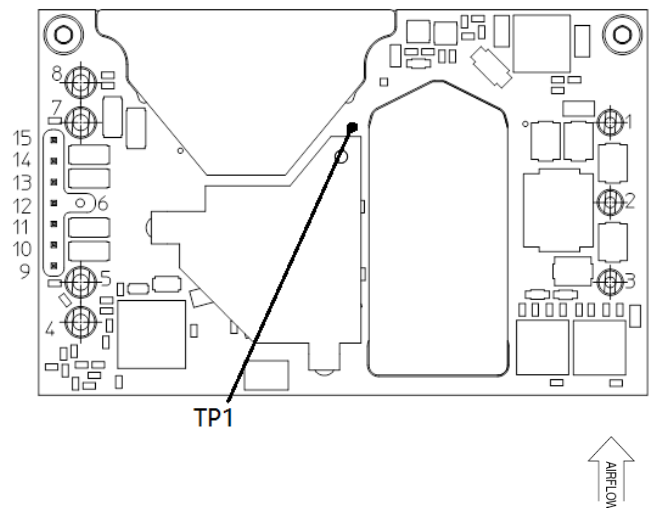
Base plate (Bottom view)
