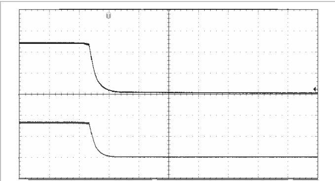
Shut-down, closed by disconnecting V_I at: T_{P1} = +25^{\circ}\text{C} , V_I = 24\text{ V} , V_O = 3.3\text{ V} I_O = 606\text{ mA} resistive load.
