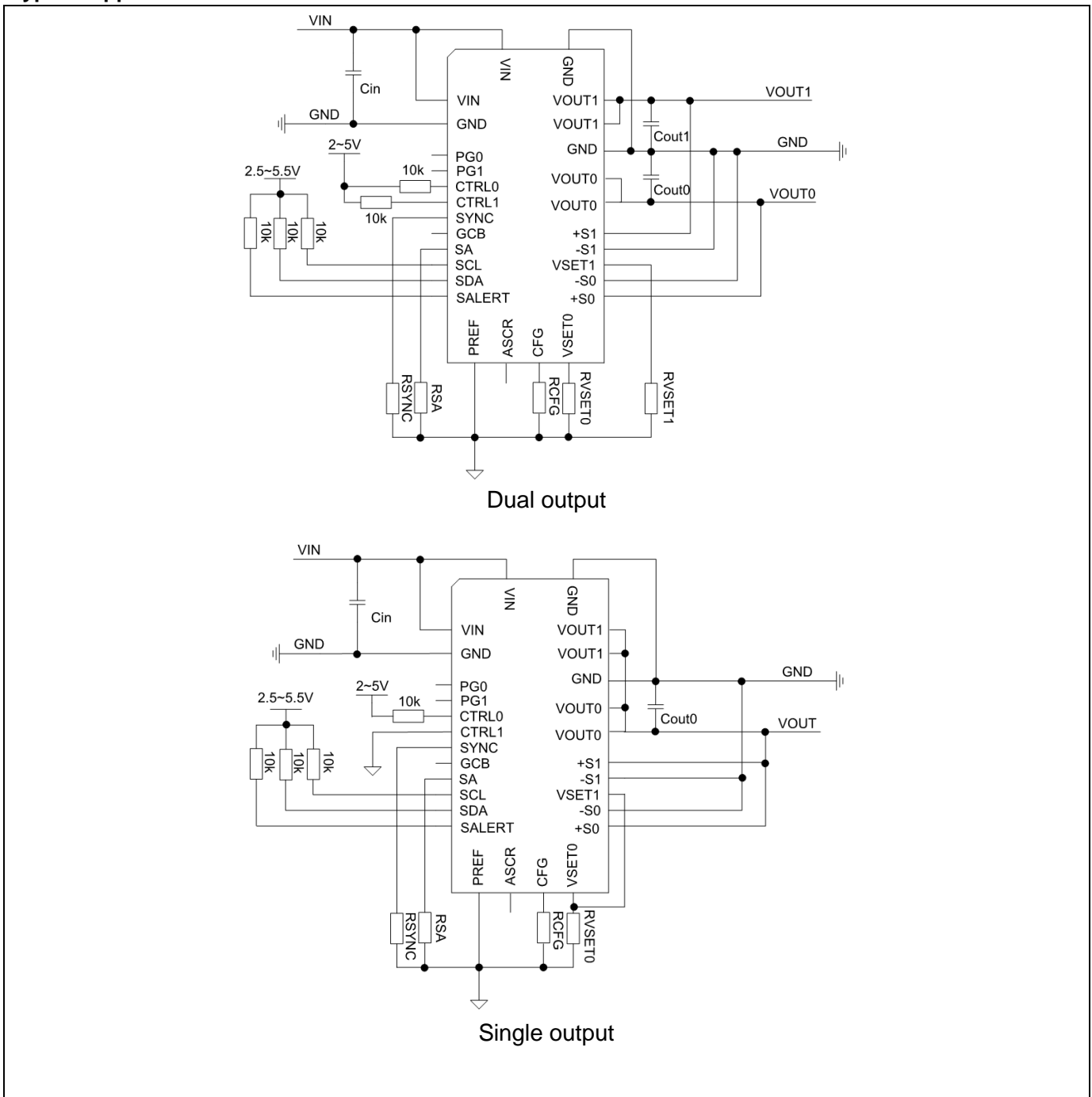
Standalone operation with PMBus communication.
