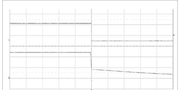
Shut-down enabled by disconnecting V_I at: T_{P1} = +25^\circ\text{C} , V_I = 48\text{ V} , I_O = 7\text{ A} resistive load. Top trace: output voltage (2 V/div.). Bottom trace: input voltage (20 V/div.). Time scale: (200 ms/div.).
