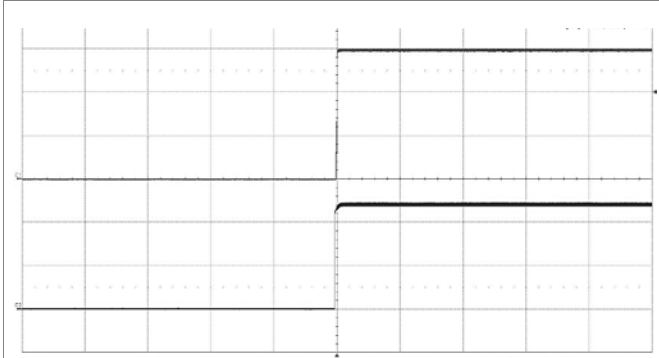
Start-up enabled by connecting V_i at: T_{P1} = +25^{\circ}\text{C} , V_i = 48\text{ V} , I_o = 2\text{ A} resistive load. Top trace: output voltage (5 V/div.). Bottom trace: input voltage (20 V/div.). Time scale: (200 ms/div.).
