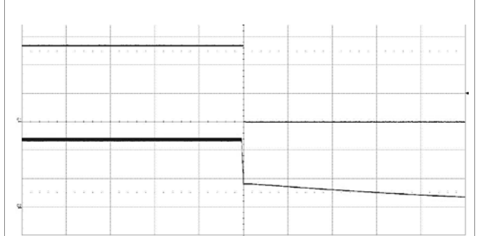
Shut-down enabled by disconnecting V_I at: T_{P1} = +25^{\circ}\text{C} , V_I = 48\text{ V} , I_O = 0.463\text{ A} resistive load. Top trace: output voltage (20 V/div.). Bottom trace: input voltage (20 V/div.). Time scale: (200 ms/div.).
