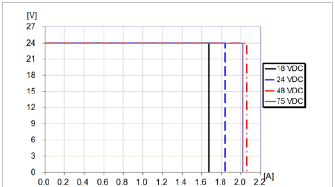
Output voltage vs. load current at I_o > \text{max } I_o at T_{P1} = +25^{\circ}\text{C} .
