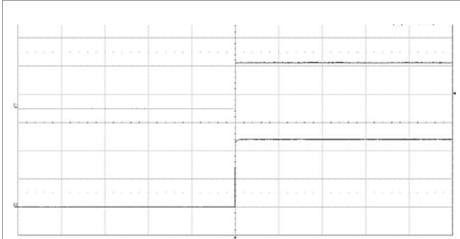
Start-up enabled by connecting V_I at: T_{P1} = +25^\circ\text{C} , V_I = 48\text{ V} , I_O = 7\text{ A} resistive load. Top trace: output voltage (2 V/div.). Bottom trace: input voltage (20 V/div.). Time scale: (200 ms/div.).
