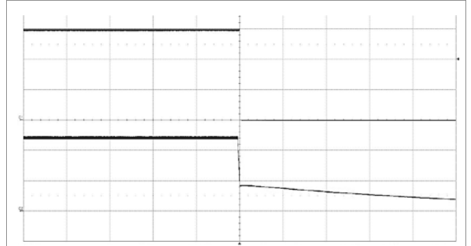
Shut-down enabled by disconnecting V_i at: T_{P1} = +25^{\circ}\text{C} , V_i = 48\text{ V} , I_o = 2\text{ A} resistive load. Top trace: output voltage (5 V/div.). Bottom trace: input voltage (20 V/div.). Time scale: (200 ms/div.).
