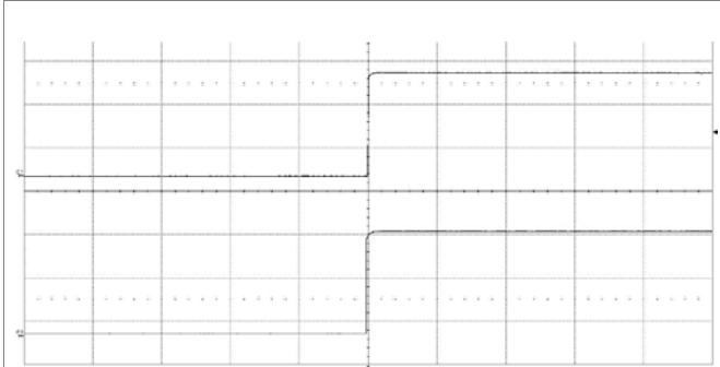
Start-up enabled by connecting V_I at: T_{P1} = +25^{\circ}\text{C} , V_I = 48\text{ V} , I_o = 0.625\text{ A} resistive load. Top trace: output voltage (20 V/div.). Bottom trace: input voltage (20 V/div.). Time scale: (200 ms/div.).
