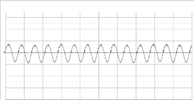
Output voltage ripple at: T_{P1} = +25^{\circ}\text{C} , V_I = 48\text{ V} , I_O = 0.463\text{ A} resistive load. Trace: output voltage (50 mV/div.). Time scale: (5 \mu\text{s} /div.). 20MHz bandwidth
