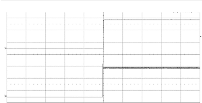
Start-up enabled by connecting V_i at: T_{P1} = +25^{\circ}\text{C} , V_i = 48\text{ V} , I_o = 1.25\text{ A} resistive load. Top trace: output voltage (10 V/div.). Bottom trace: input voltage (20 V/div.). Time scale: (200 ms/div.).
