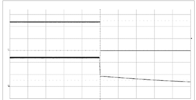
Shut-down enabled by disconnecting V_I at: T_{P1} = +25^{\circ}\text{C} , V_I = 48\text{ V} , I_o = 2.5\text{ A} resistive load. Top trace: output voltage (5 V/div.). Bottom trace: input voltage (20 V/div.). Time scale: (200 ms/div.).
