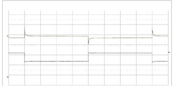
Output voltage response to load current step- change (3.5-5.25-3.5 A) at: T_{P1} = +25^\circ\text{C} , V_I = 48\text{ V} . Top trace: output voltage (200 mV/div.). Bottom trace: load current (2 A/div.). Time scale: (2 ms/div.).
