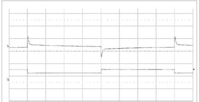
Output voltage response to load current step-change (0.312-0.468-0.312 A) at: T_{P1} = +25^{\circ}\text{C} , V_I = 48\text{ V} . Top trace: output voltage (500 mV/div.). Bottom trace: load current (500 mA/div.). Time scale: (2 ms/div.).
