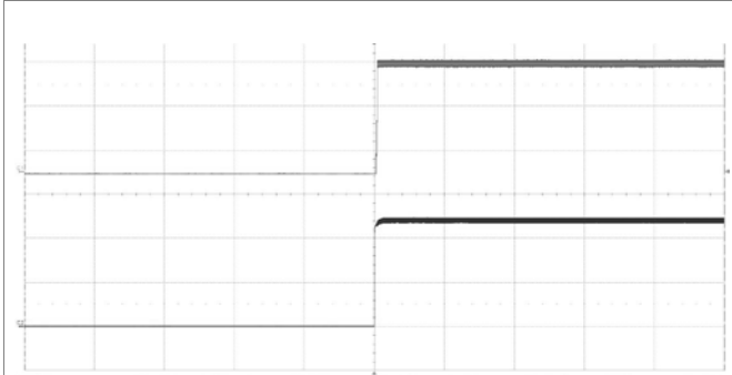
Start-up enabled by connecting V_I at: T_{P1} = +25^{\circ}\text{C} , V_I = 48\text{ V} , I_o = 6\text{ A} resistive load. Top trace: output voltage (2 V/div.). Bottom trace: input voltage (20 V/div.). Time scale: (200 ms/div.).
