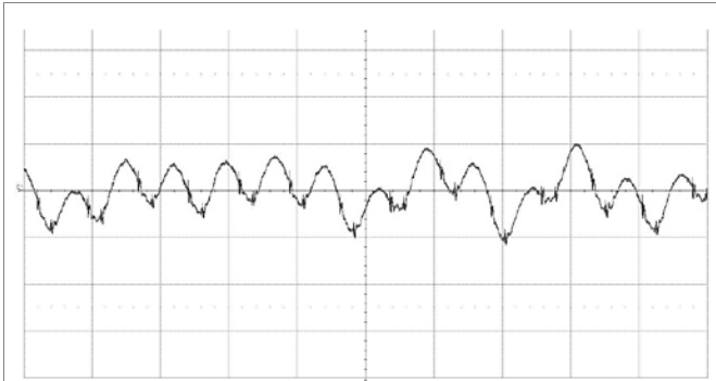
Output voltage ripple at: T_{P1} = +25^{\circ}\text{C} , V_i = 48\text{ V} , I_o = 2\text{ A} resistive load. Trace: output voltage (20 mV/div.). Time scale: (5 \mu\text{s} /div.). 20MHz bandwidth
