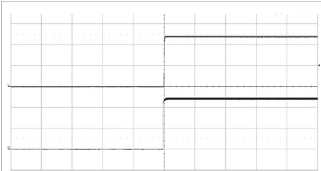
Start-up enabled by connecting V_I at: T_{P1} = +25^{\circ}\text{C} , V_I = 48\text{ V} , I_o = 2.5\text{ A} resistive load. Top trace: output voltage (5 V/div.). Bottom trace: input voltage (20 V/div.). Time scale: (200 ms/div.).
