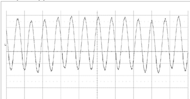
Output voltage ripple at: T_{P1} = +25^{\circ}\text{C} , V_i = 24\text{ V} , I_o = 1.25\text{ A} resistive load. Trace: output voltage (10 mV/div.). Time scale: (5 \mu\text{s} /div.). 20MHz bandwidth
