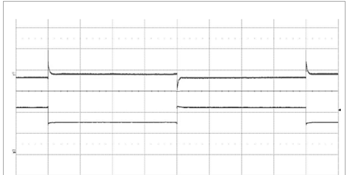
Output voltage response to load current step-change (3.0-4.5-3.0 A) at: T_{P1} = +25^{\circ}\text{C} , V_I = 48\text{ V} . Top trace: output voltage (200 mV/div.). Bottom trace: load current (2 A/div.). Time scale: (2 ms/div.).
