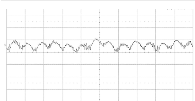
Output voltage ripple at: T_{P1} = +25^\circ\text{C} , V_I = 48\text{ V} , I_O = 7\text{ A} resistive load. Trace: output voltage (10 mV/div.). Time scale: (5 μs/div.). 20MHz bandwidth
