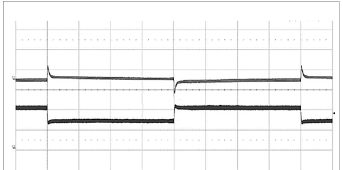
Output voltage response to load current step-change (0.231-0.347-0.231 A) at: T_{P1} = +25^{\circ}\text{C} , V_I = 48\text{ V} . Top trace: output voltage (500 mV/div.). Bottom trace: load current (200 mA/div.). Time scale: (2 ms/div.).
