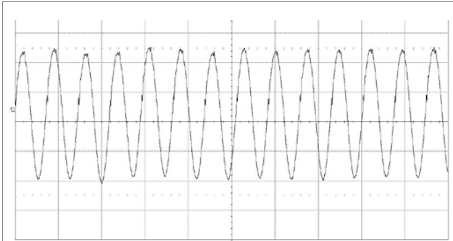
Output voltage ripple at: T_{P1} = +25^{\circ}\text{C} , V_I = 48\text{ V} , I_o = 0.625\text{ A} resistive load. Trace: output voltage (20 mV/div.). Time scale: (5 \mu\text{s} /div.). 20MHz bandwidth
