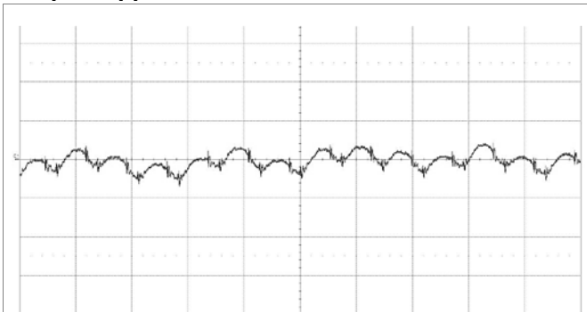
Output voltage ripple at: T_{P1} = +25^{\circ}\text{C} , V_I = 48\text{ V} , I_o = 2.5\text{ A} resistive load. Trace: output voltage (20 mV/div.). Time scale: (5 μs/div.). 20MHz bandwidth
