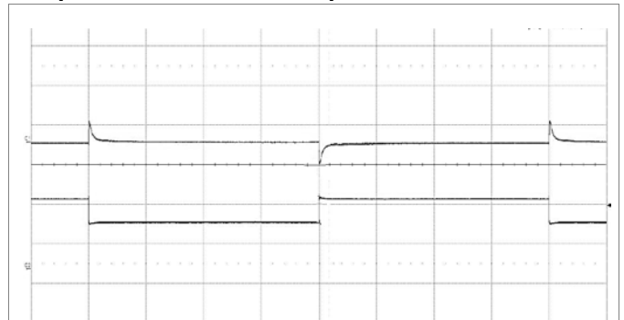
Output voltage response to load current step-change (1.25-1.875-1.25 A) at: T_{P1} = +25^{\circ}\text{C} , V_I = 48\text{ V} . Top trace: output voltage (500 mV/div.). Bottom trace: load current (1 A/div.). Time scale: (2 ms/div.).
