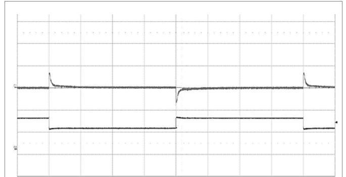
Output voltage response to load current step-change (1.0-1.5-1.0 A) at: T_{P1} = +25^{\circ}\text{C} , V_i = 48\text{ V} . Top trace: output voltage (500 mV/div.). Bottom trace: load current (1 A/div.). Time scale: (2 ms/div.).
