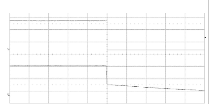
Shut-down enabled by disconnecting V_I at: T_{P1} = +25^{\circ}\text{C} , V_I = 48\text{ V} , I_o = 0.625\text{ A} resistive load. Top trace: output voltage (20 V/div.). Bottom trace: input voltage (20 V/div.). Time scale: (200 ms/div.).
