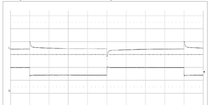
Output voltage response to load current step- change (0.625-0.937-0.625 A) at: T_{P1} = +25^{\circ}\text{C} , V_i = 24\text{ V} . Top trace: output voltage (500 mV/div.). Bottom trace: load current (500 mA/div.). Time scale: (2 ms/div.).
