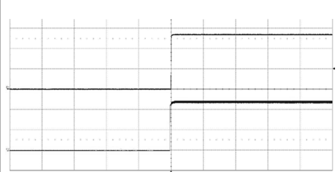
Start-up enabled by connecting V_I at: T_{P1} = +25^{\circ}\text{C} , V_I = 48\text{ V} , I_O = 0.463\text{ A} resistive load. Top trace: output voltage (20 V/div.). Bottom trace: input voltage (20 V/div.). Time scale: (200 ms/div.).
