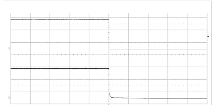
Output disabled by removing V_i at: T_{P1} = +25^{\circ}\text{C} , V_i = 48\text{ V} , I_o = 1.25\text{ A} resistive load. Top trace: output voltage (10 V/div.). Bottom trace: input voltage (20 V/div.). Time scale: (200 ms/div.).
