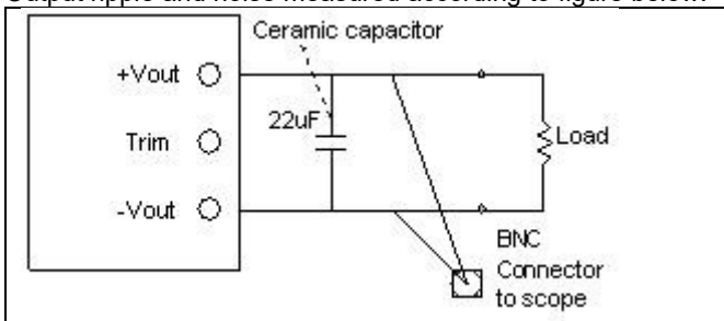
Output ripple and noise test setup for PKE 53XX variants
