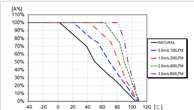
Available load current vs. ambient air temperature and airflow at V_I = 24\text{ V} . See Thermal Consideration section.
