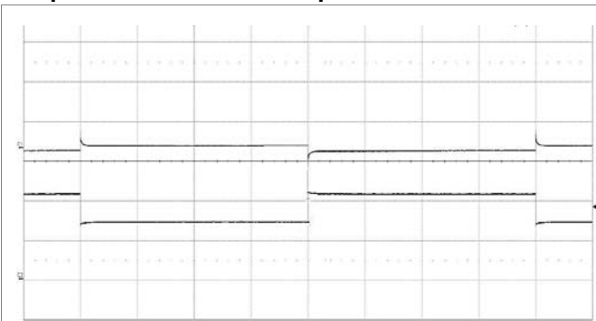
Output voltage response to load current step-change (3.0-4.5-3.0 A) at: T_{P1} = +25^{\circ}\text{C} , V_I = 24\text{ V} . Top trace: output voltage (500 mV/div.). Bottom trace: load current (2 A/div.). Time scale: (2 ms/div.).
