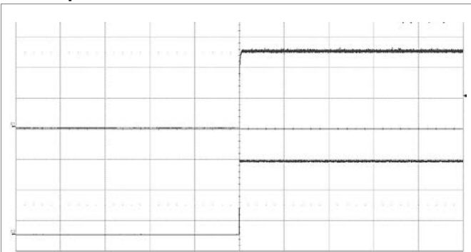
Start-up enabled by connecting V_I at: T_{P1} = +25^{\circ}\text{C} , V_I = 24\text{ V} , I_O = 6\text{ A} resistive load. Top trace: output voltage (2 V/div.). Bottom trace: input voltage (10 V/div.). Time scale: (200 ms/div.).
