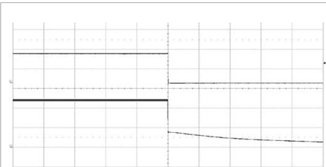
Output disabled by removing V_I at: T_{P1} = +25^{\circ}\text{C} , V_I = 24\text{ V} , I_O = 2\text{ A} resistive load. Top trace: output voltage (10 V/div.). Bottom trace: input voltage (10 V/div.). Time scale: (200 ms/div.).
