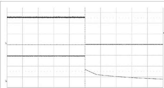
Output voltage disabled by removing V_I at: T_{P1} = +25^{\circ}\text{C} , V_I = 24\text{ V} , I_O = 6\text{ A} resistive load. Top trace: output voltage (2 V/div.). Bottom trace: input voltage (10 V/div.). Time scale: (200 ms/div.).
