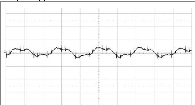
Output voltage ripple at: T_{P1} = +25^{\circ}\text{C} , V_I = 24\text{ V} , I_O = 6\text{ A} resistive load. Trace: output voltage (20 mV/div.). Time scale: (5 \mu\text{s} /div.) 20 MHz bandwidth
