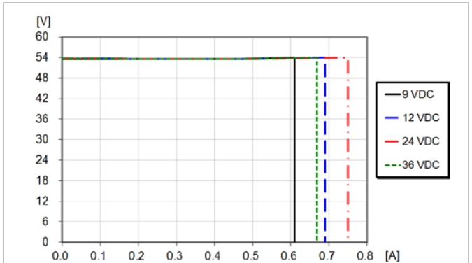
Output voltage vs. load current at I_O > \max I_O at T_{P1} = +25^{\circ}\text{C} .
