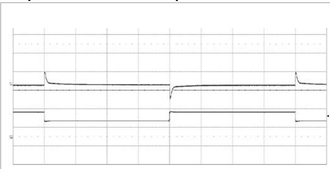
Output voltage response to load current step- change (1.0-1.5-1.0 A) at: T_{P1} = +25^{\circ}\text{C} , V_I = 24\text{ V} . Top trace: output voltage (500 mV/div.). Bottom trace: load current (1 A/div.). Time scale: (2 ms/div.).
