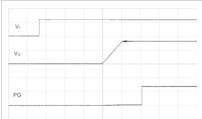
Start-up enabled by applying V_i . T_{ON\_DELAY} = T_{ON\_RISE} = 10\text{ ms} (default). V_i = 12\text{ V} , I_o = \text{max } I_o , PG pulled up to V_o . Scale: 10 or 2 V/div, 10 ms/div.
