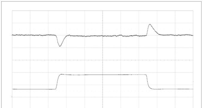
Output voltage response to load current step change (3–9 A) at V_i = 12\text{ V} , C_o = 3 \times 100\ \mu\text{F} + 270\ \mu\text{F}/10\text{m}\Omega . Default compensation settings. Scale: 50 mV/div, 5 A/div, 50 \mu\text{s} /div.
