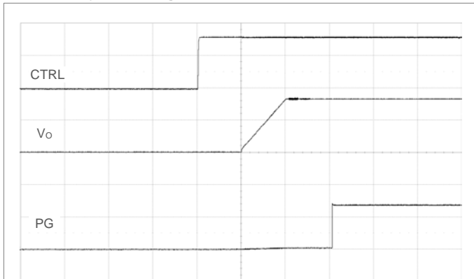
Start-up enabled by CTRL signal. T_{ON\_DELAY} = T_{ON\_RISE} = 10\text{ ms} (default). V_i = 12\text{ V} , I_o = \text{max } I_o , PG pulled up to V_o . Scale: 2 V/div, 10 ms/div.
