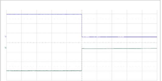
Shut-down enabled by disconnecting V_I at: T_{P1} = +25^\circ\text{C}, V_I = 24\text{ V}, I_O = +0.625\text{ A} resistive load. Top trace: output1 voltage (5 V/div.). Bottom trace: output2 voltage (5 V/div.). Time scale: (200 ms/div.).
