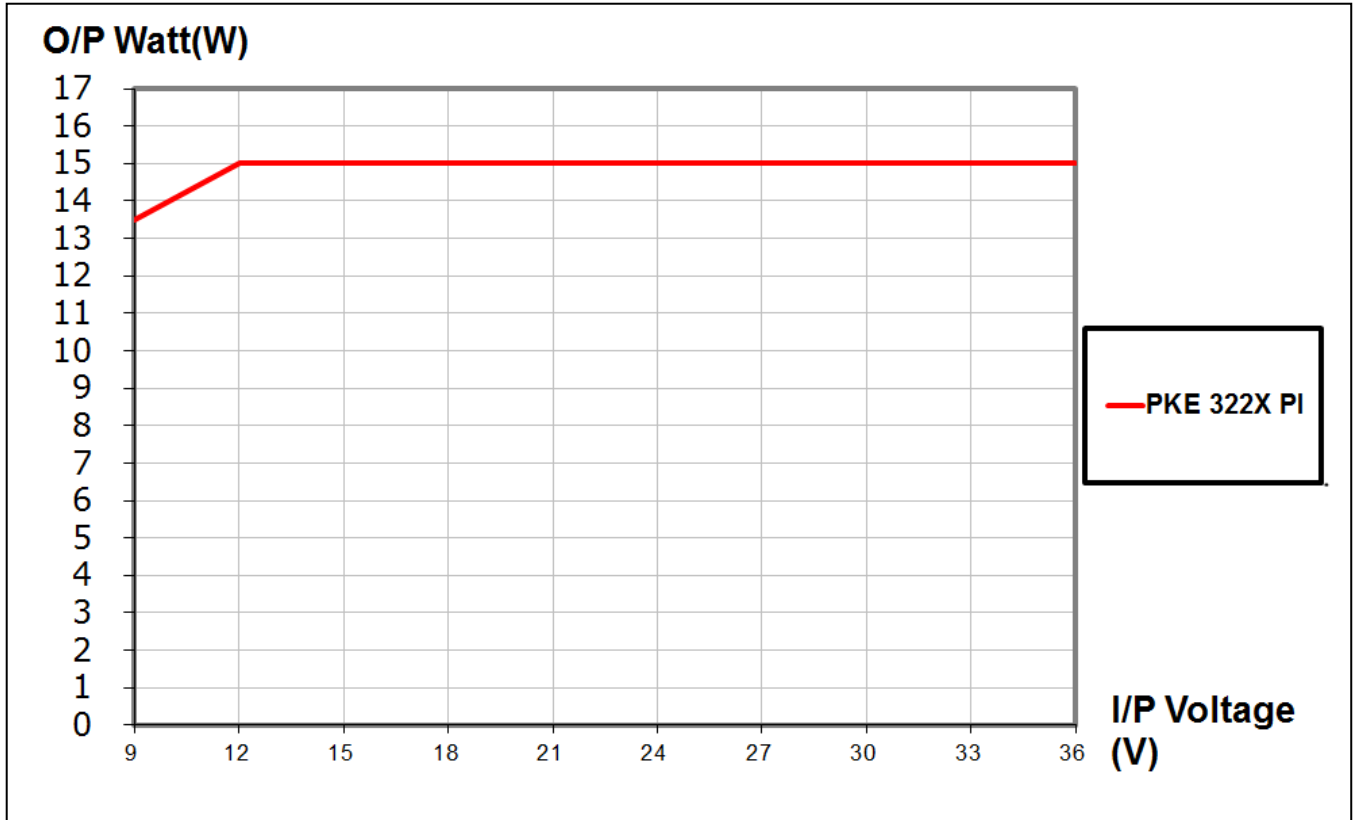
Note 4: PKE 3221 PI Power Derating Curve (Output Power VS Input Voltage)
