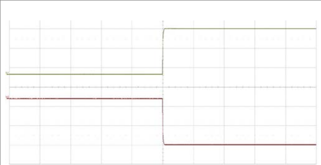
Start-up enabled by connecting V_I at: T_{P1} = +25^\circ\text{C}, V_I = 24\text{ V}, I_O = +0.625\text{ A} resistive load. Top trace: output1 voltage (5 V/div.). Bottom trace: output2 voltage (5 V/div.). Time scale: (200 ms/div.).
