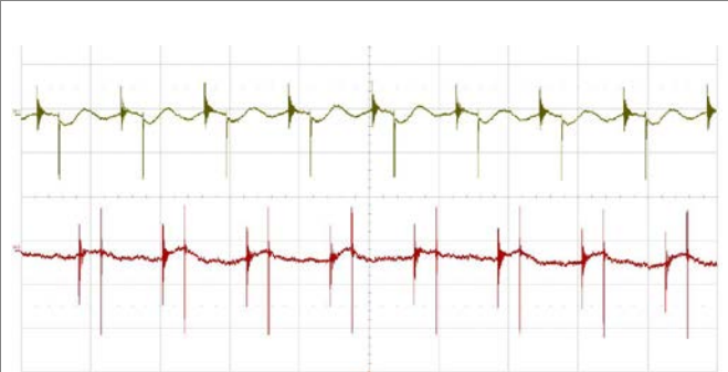
Output voltage ripple at: T_{P1} = +25^\circ\text{C}, V_I = 24\text{ V}, I_O = +0.625\text{ A} resistive load. Trace: output voltage (10 mV/div.). Time scale: (5 \mu\text{s} /div.). 20MHz bandwidth
