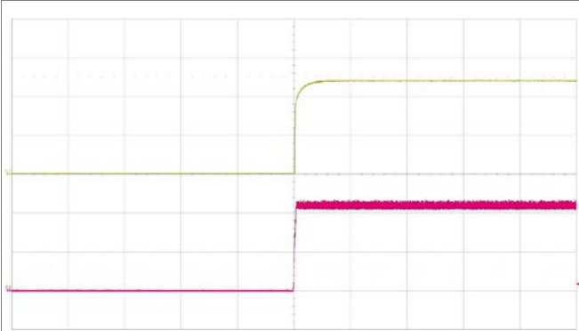
Start-up enabled by connecting V_I at: T_{P1} = +25^{\circ}\text{C} , V_I = 110\text{ V} , I_O = 8.4\text{ A} resistive load. Top trace: output voltage (10 V/div.). Bottom trace: input voltage (50 V/div.). Time scale: (200 ms/div.).
