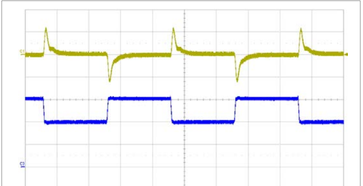
Output voltage response to load current step-change (6.3-4.2-6.3 A) at: T_{P1} = +25^{\circ}\text{C} , V_I = 110\text{ V} . Top trace: output voltage (500mV/div.). Bottom trace: load current (2 A/div.). Time scale: (500 \mu\text{s} /div.).
