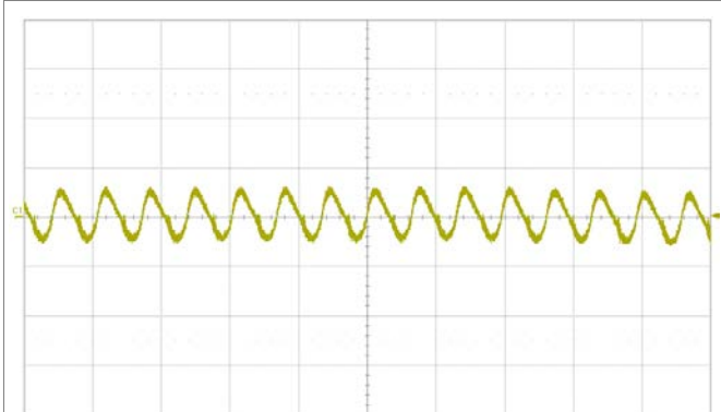
Output voltage ripple at: T_{P1} = +25^{\circ}\text{C} , V_I = 110\text{ V} , I_O = 4.2\text{ A} resistive load. Trace: output voltage (100 mV/div.). Time scale: (5 \mu\text{s} /div.). 20 MHz bandwidth.
