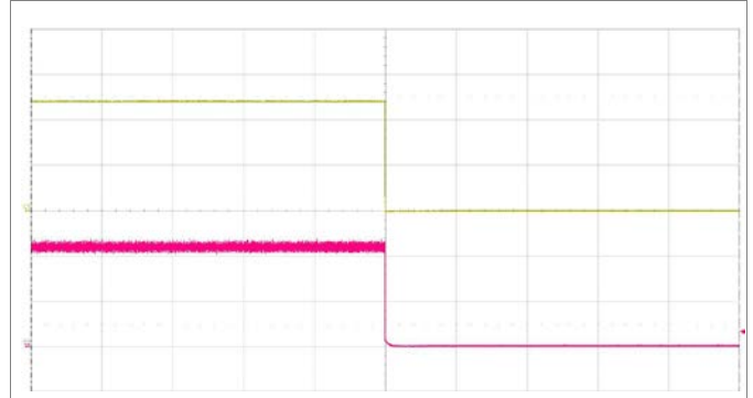
Shut-down enabled by disconnecting V_I at: T_{P1} = +25^{\circ}\text{C} , V_I = 110\text{ V} , I_O = 4.2\text{ A} resistive load. Top trace: output voltage (20 V/div.). Bottom trace: input voltage (50 V/div.). Time scale: (500 ms/div.).
