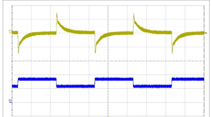
Output voltage response to load current step- change (2.1-3.15-2.1 A) at: T_{P1} = +25^{\circ}\text{C} , V_I = 110\text{ V} . Top trace: output voltage (500 mV/div.). Bottom trace: load current (2 A/div.). Time scale: (500 \mu\text{s} /div.).
