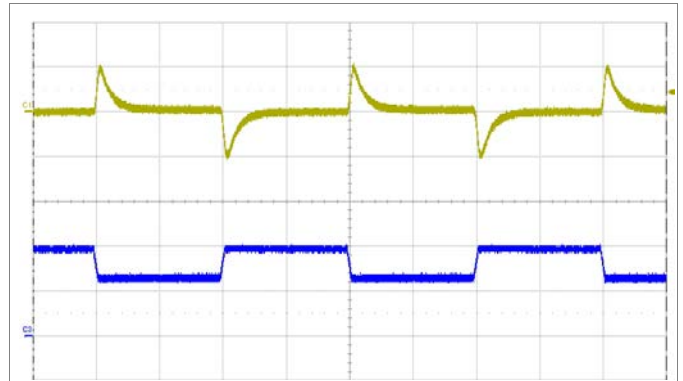
Output voltage response to load current step-change (6.75-10.125-6.75 A) at: T_{P1} = +25^{\circ}\text{C} , V_I = 110\text{ V} . Top trace: output voltage (500 mV/div.). Bottom trace: load current (5 A/div.). Time scale: (500 \mu\text{s} /div.).
