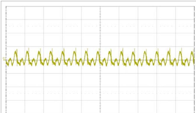
Output voltage ripple at: T_{P1} = +25^{\circ}\text{C} , V_I = 110\text{ V} , I_O = 13.5\text{ A} resistive load. Trace: output voltage (20 mV/div.). Time scale: (5 \mu\text{s} /div.). 20 MHz bandwidth.
