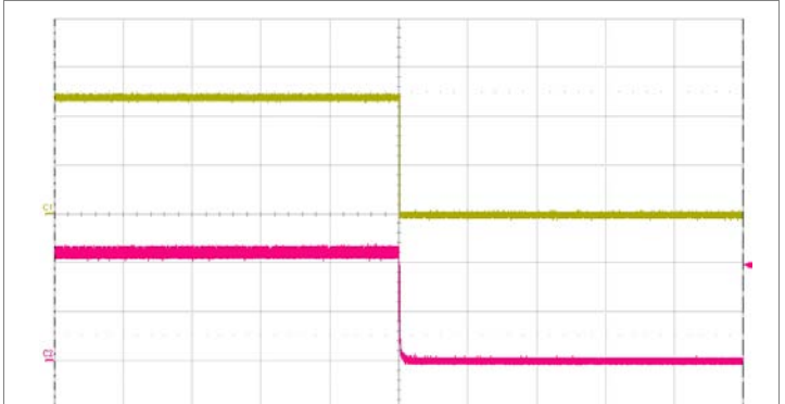
Shut-down enabled by disconnecting V_I at: T_{P1} = +25^{\circ}\text{C} , V_I = 110\text{ V} , I_O = 8.4\text{ A} resistive load. Top trace: output voltage (10 V/div.). Bottom trace: input voltage (50 V/div.). Time scale: (200 ms/div.).
