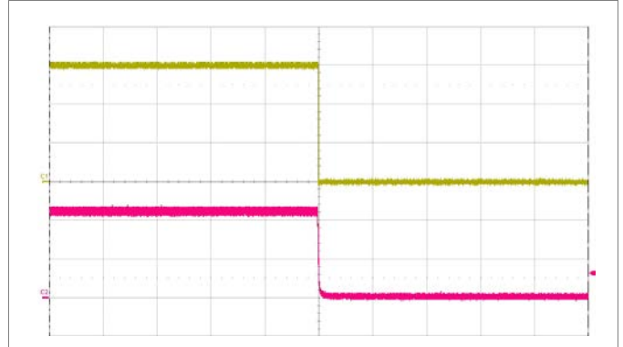
Shut-down enabled by disconnecting V_I at: T_{P1} = +25^{\circ}\text{C} , V_I = 110\text{ V} , I_O = 13.5\text{ A} resistive load. Top trace: output voltage (5 V/div.). Bottom trace: input voltage (50 V/div.). Time scale: (500 ms/div.).
