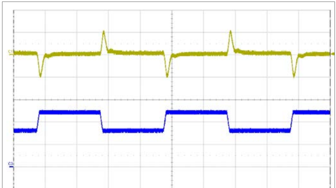
Output voltage response to load current step- change (8.4-12.6-8.4 A) at: T_{P1} = +25^{\circ}\text{C} , V_I = 110\text{ V} . Top trace: output voltage (500 mV/div.). Bottom trace: load current (5 A/div.). Time scale: (500 \mu\text{s} /div.).
