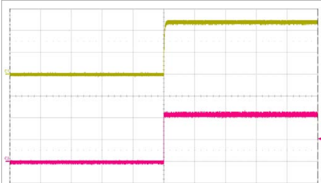
Start-up enabled by connecting V_I at: T_{P1} = +25^{\circ}\text{C} , V_I = 110\text{ V} , I_O = 16.8\text{ A} resistive load. Top trace: output voltage (5V/div.). Bottom trace: input voltage (50 V/div.). Time scale: (500 ms/div.).
