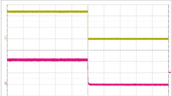
Shut-down enabled by disconnecting V_I at: T_{P1} = +25^{\circ}\text{C} , V_I = 110\text{ V} , I_O = 16.8\text{ A} resistive load. Top trace: output voltage (5 V/div.). Bottom trace: input voltage (50 V/div.). Time scale: (500 ms/div.).
