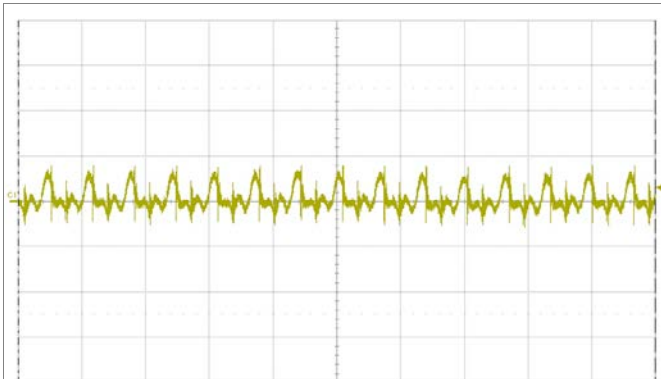
Output voltage ripple at: T_{P1} = +25^{\circ}\text{C} , V_I = 110\text{ V} , I_O = 16.8\text{ A} resistive load. Trace: output voltage (20 mV/div.). Time scale: (5 \mu\text{s} /div.). 20 MHz bandwidth.
