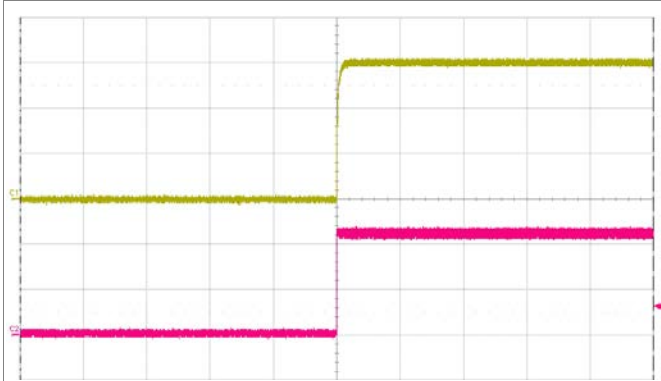
Start-up enabled by connecting V_I at: T_{P1} = +25^{\circ}\text{C} , V_I = 110\text{ V} , I_O = 13.5\text{ A} resistive load. Top trace: output voltage (5 V/div.). Bottom trace: input voltage (50 V/div.). Time scale: (500 ms/div.).
