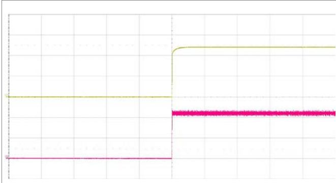
Start-up enabled by connecting V_I at: T_{P1} = +25^{\circ}\text{C} , V_I = 110\text{ V} , I_O = 4.2\text{ A} resistive load. Top trace: output voltage (20 V/div.). Bottom trace: input voltage (50 V/div.). Time scale: (500 ms/div.).
