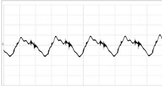
Output voltage ripple at: T_{P1} = +25^\circ\text{C} , V_i = 53\text{ V} , I_o = 96.2\text{ A} resistive load. Trace: output voltage 20 mV/div. Time scale: 2 \mu\text{s} /div.
