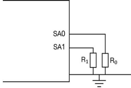
Schematic of connection of address resistors, (SA0 is not used in the 4 pin digital header variant)
