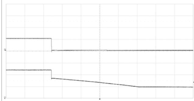
Shut-down enabled by disconnecting V_i at: T_{P1} = +25^\circ\text{C} , V_i = 53\text{ V} , I_o = 96.2\text{ A} resistive. Top trace: output voltage 10 V/div. Bottom trace: div input voltage 20 V/div. Time scale: 50 ms/div.
