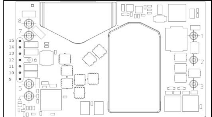
Connections (Bottom view)
