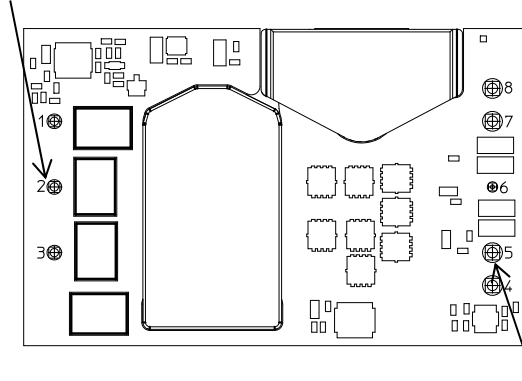
Pin 5 for measurement of minimum pin (solder joint) temperature, T_{PIN}
