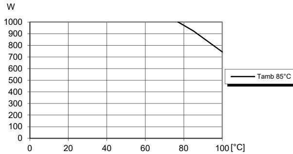
Available load current vs. base plate temperature. V_i = 53 V. See Thermal Consideration section.
