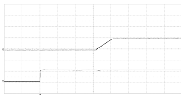
Start-up enabled by connecting V_i at: T_{P1} = +25^\circ\text{C} , V_i = 53\text{ V} , I_o = 96.2\text{ A} resistive load. Top trace: output voltage 10 V/div. Bottom trace: input voltage 50 V/div. Time scale: 10 ms/div
