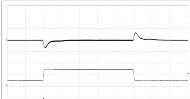
Output voltage response to load current step- change 24-72-24 A (2 A/ \mu\text{s} ) at: T_{P1} = +25^\circ\text{C} , V_i = 53\text{ V} . Top trace: output voltage 500 mV/div. Bottom trace: load current 50 A/div. Time scale: 0.5 ms/div.
