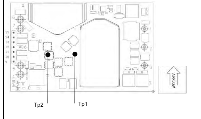
Base plate (Bottom view)
