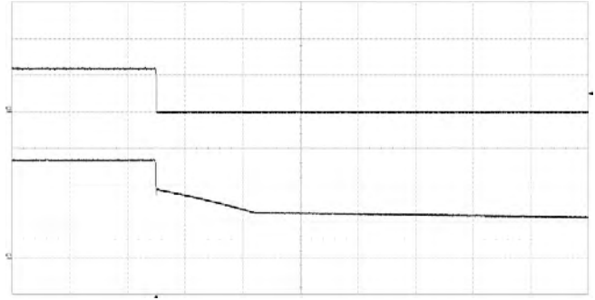
Shut-down enabled by disconnecting V_i at: T_{PI} = +25^\circ\text{C} , V_i = 53\text{ V} , I_o = 75\text{ A} resistive load.
