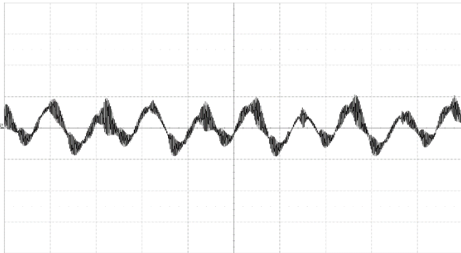
Output voltage ripple at: T_{PI} = +25^\circ\text{C} , V_i = 53\text{ V} , I_o = 220\text{ A} resistive load.
