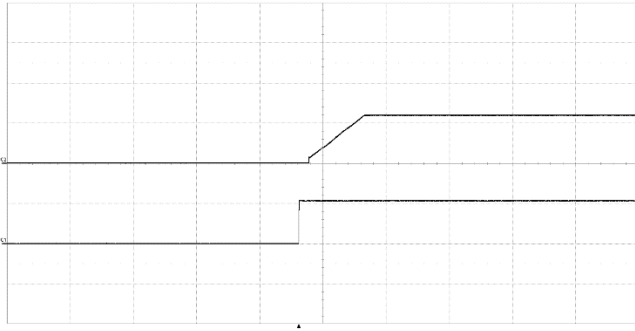
Start-up enabled by connecting V_i at: T_{PI} = +25^\circ\text{C} , V_i = 53\text{ V} , I_o = 75\text{ A} resistive load.
