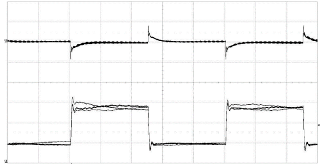
Output voltage response to load current step- change 56-168-56 A (2 A/ \mu\text{s} ) at: T_{PI} = +25^\circ\text{C} , V_i = 53\text{ V} .
