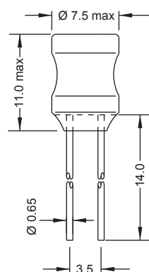
Loose / Box [-50]
