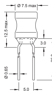
Taped / Reel [-51]
